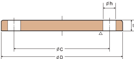
NOMINAL SIZE 10A-600A
