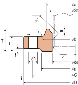
A TYPE : NOMINAL SIZE 10A-400A
