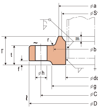
A TYPE : NOMINAL SIZE 10A-600A
