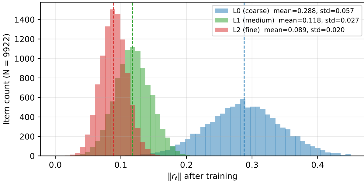
Per-layer residual norm distribution (seed=42)
