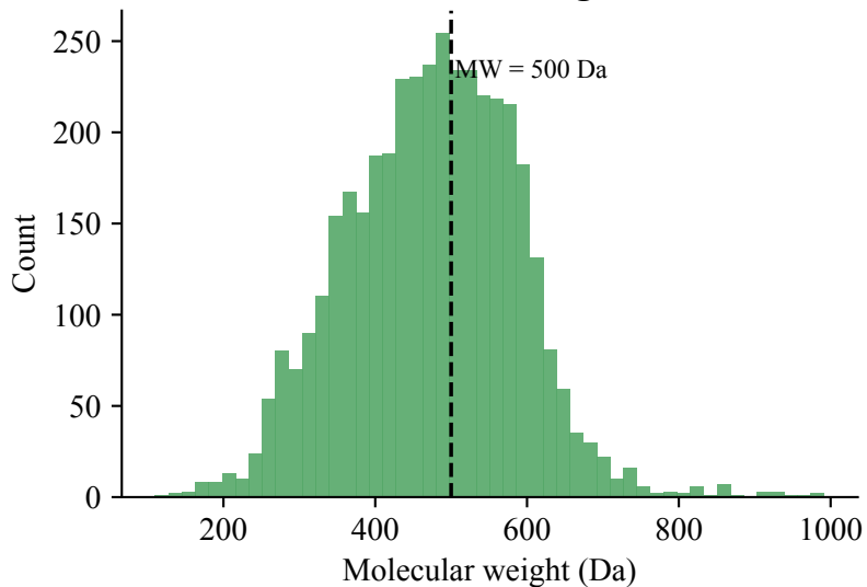
Molecular Weight
