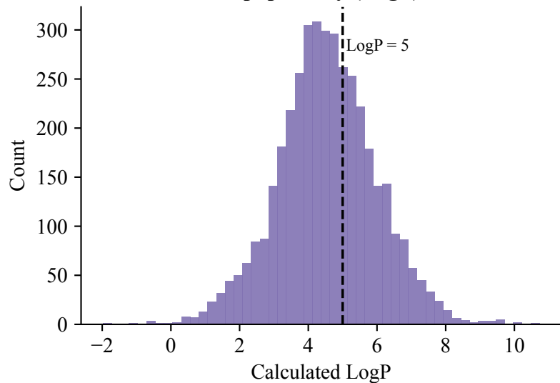
Lipophilicity (LogP)
