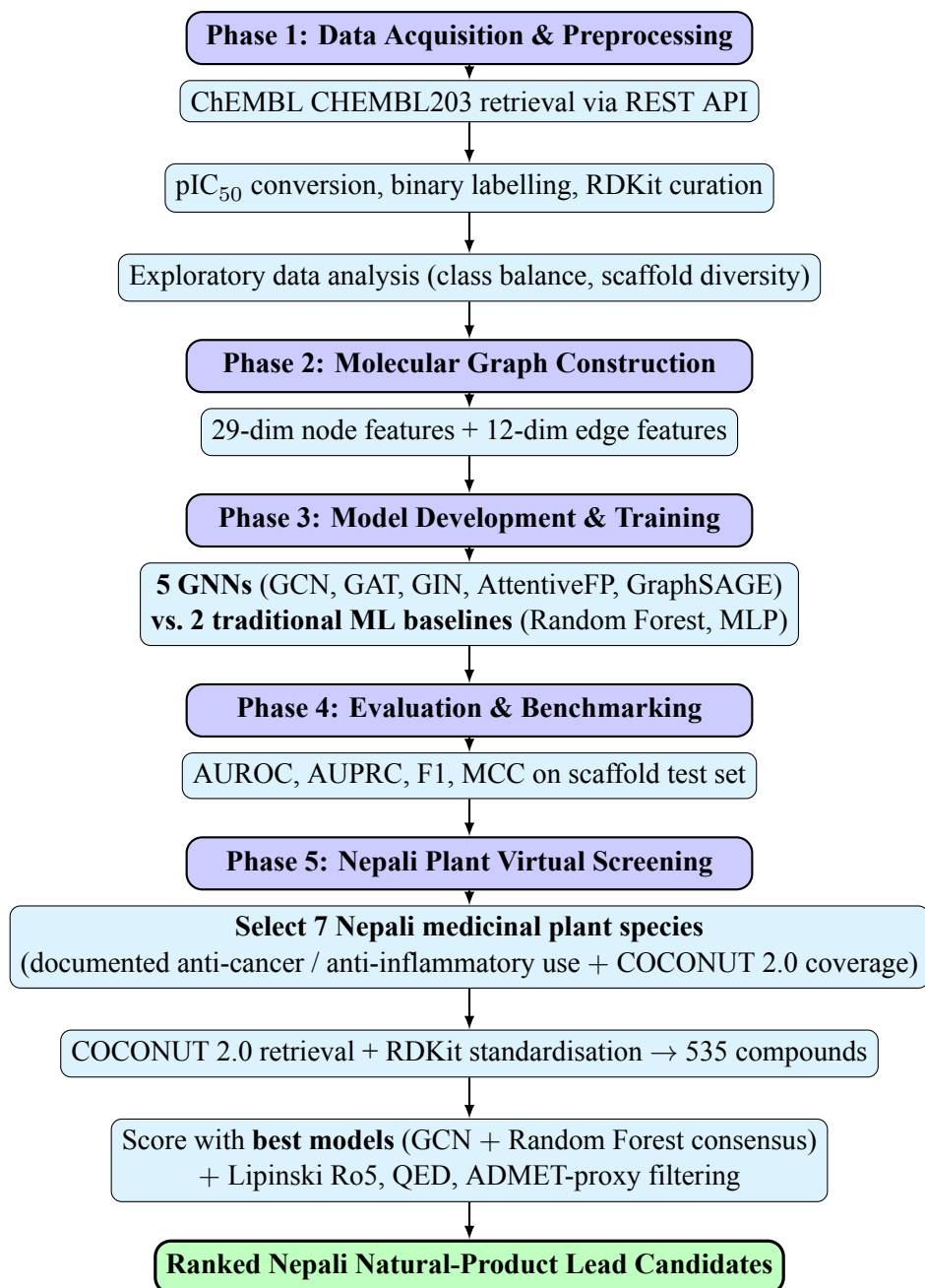
Figure 3: Five-phase computational pipeline: benchmarking five GNN architectures against traditional machine-learning baselines for EGFR inhibitor classification, and deploying the best-performing models (GCN and Random Forest) to screen a Nepali medicinal-plant compound library—whose seven species were selected by documented anti-cancer use and COCONUT 2.0 coverage.
