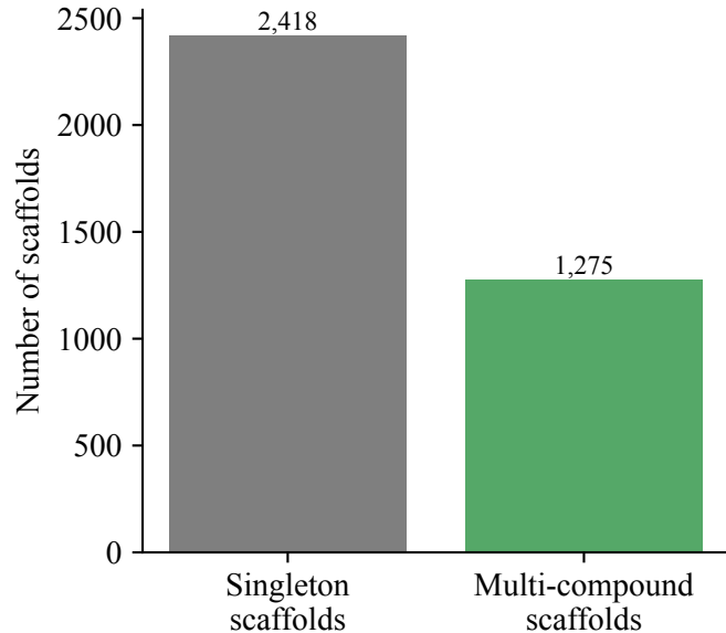
Scaffold Diversity (3,693 unique scaffolds)
