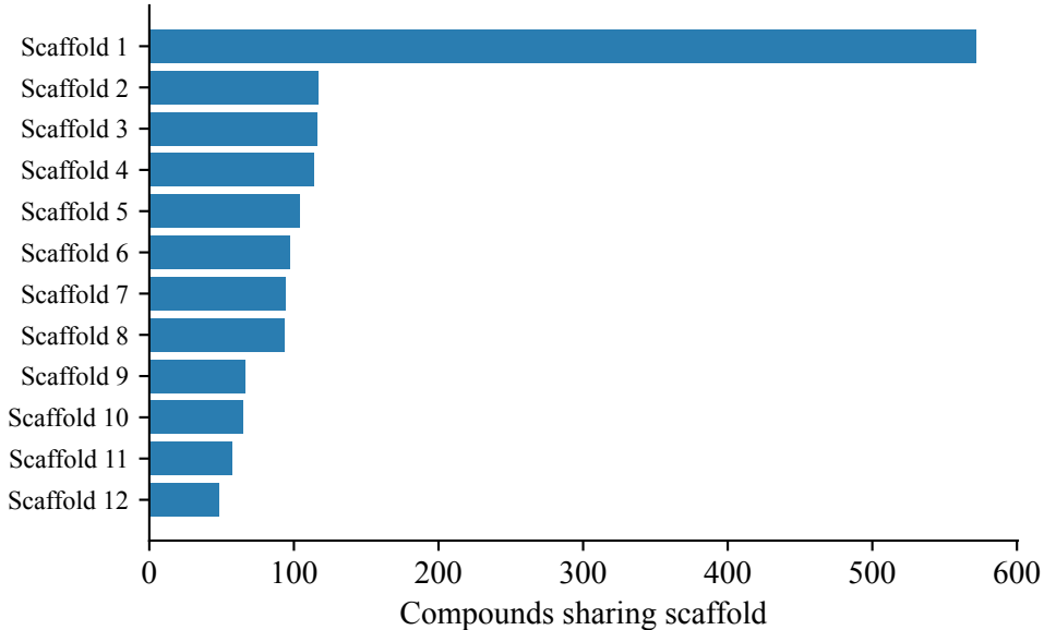
12 Most Frequent Murcko Scaffolds
