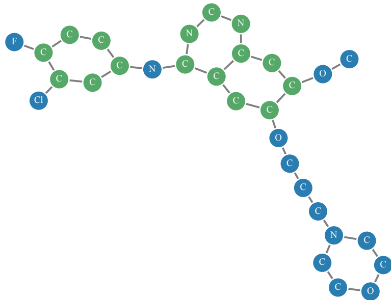
(b) Attributed molecular graph
