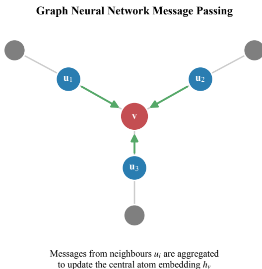
Figure 2: One step of graph neural network message passing. The central atom v updates its representation by aggregating learned messages from its bonded neighbours u_1, u_2, u_3 . Repeating this over several layers lets each atom’s embedding incorporate progressively larger chemical neighbourhoods.
