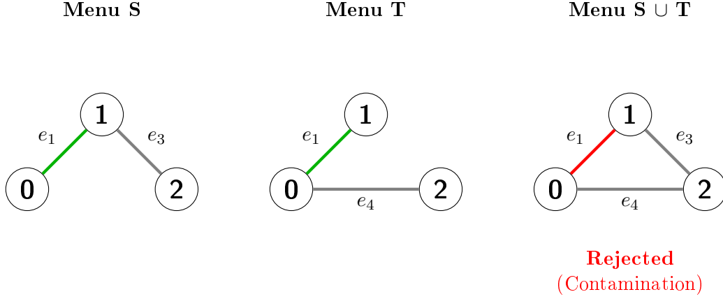
Figure 3: Geometric \gamma -Violation: Edge e_1 is choiceworthy (green) in menus S and T individually because no alternative closed path exists. In the union S \cup T , the edges e_3 and e_4 close a topological triangle. e_1 is recognized as an inefficient shortcut (contamination) and is rejected (red) by the projector.
