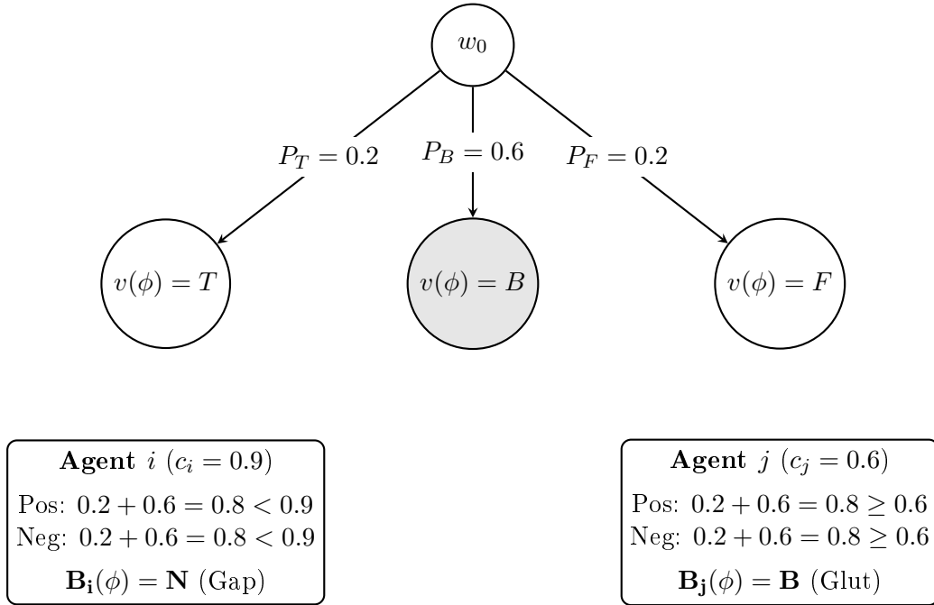
Figure 4: Multi-Agent Disagreement over a Kripke Model. Two agents ( i and j ) share the same local measure from w_0 but apply different Lockean thresholds. The same objective evidence evaluates to an Epistemic Gap ( N ) for the risk-averse Agent i , and an Epistemic Glut ( B ) for the permissive Agent j .
