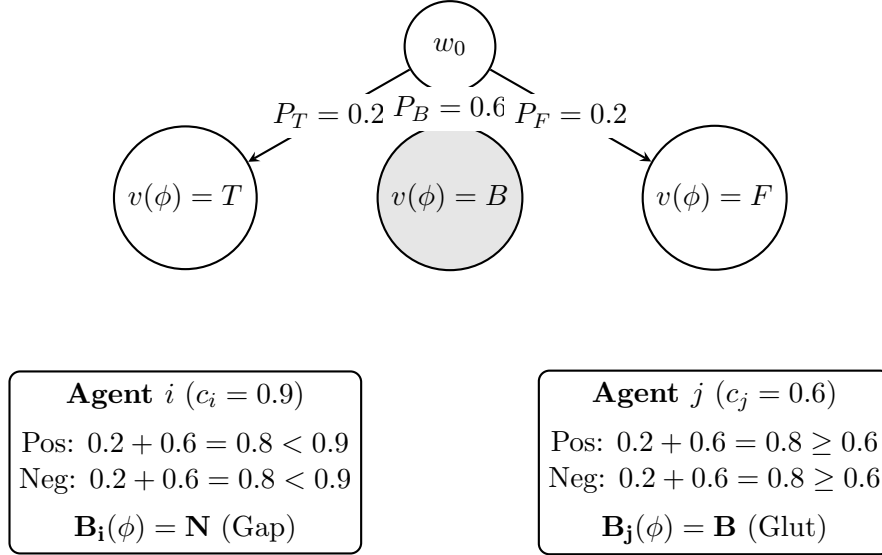
Figure 3: Multi-Agent Disagreement over a Kripke Model. Two agents ( i and j ) share the same local measure from w_0 but apply different Lockean thresholds. The same objective evidence evaluates to an Epistemic Gap ( N ) for the risk-averse Agent i , and an Epistemic Glut ( B ) for the permissive Agent j .
