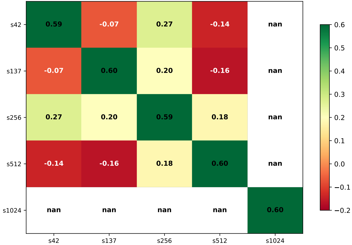
C. Connectivity (min r on path)
