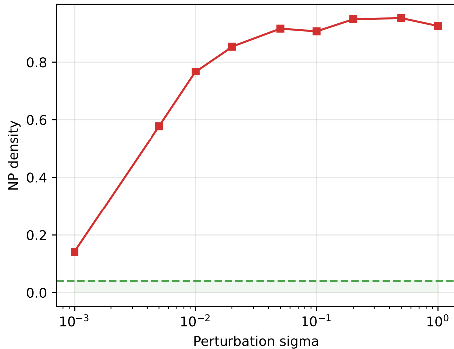
B. NP density under perturbation
