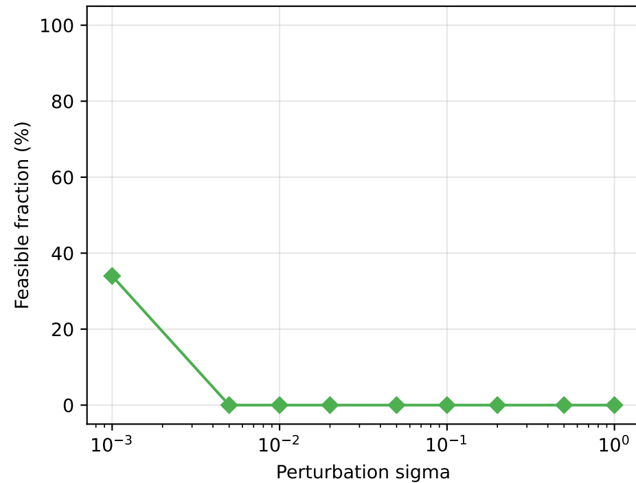
C. Basin feasibility radius
