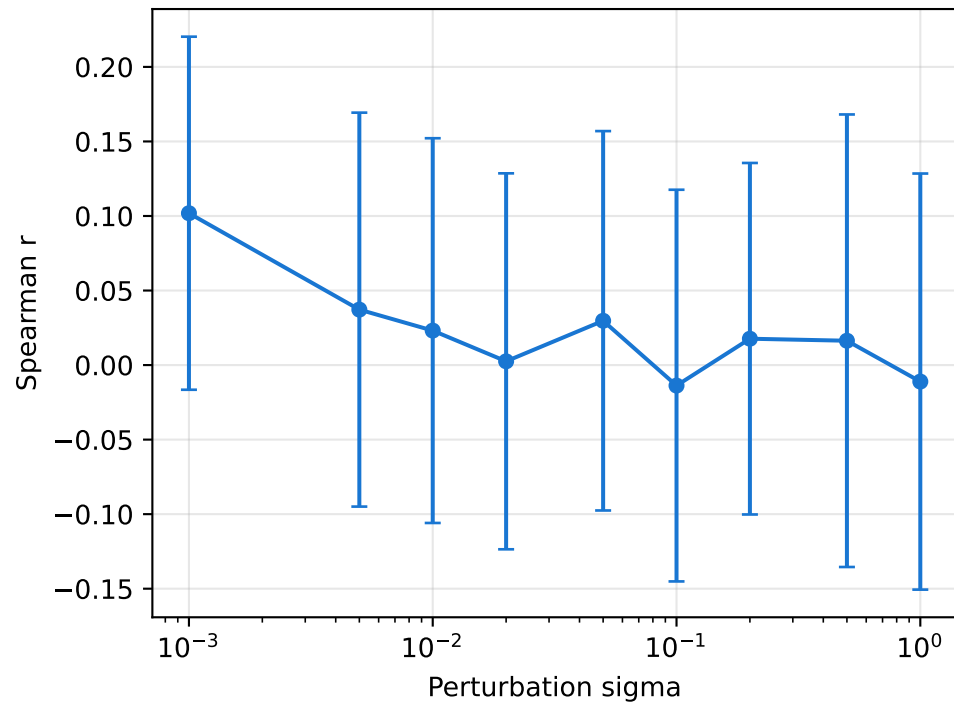
A. Prediction stability
