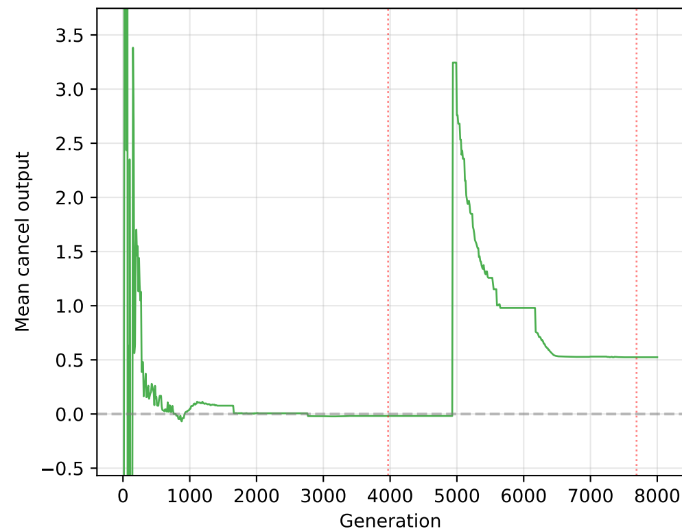
D. Cancellation residual
