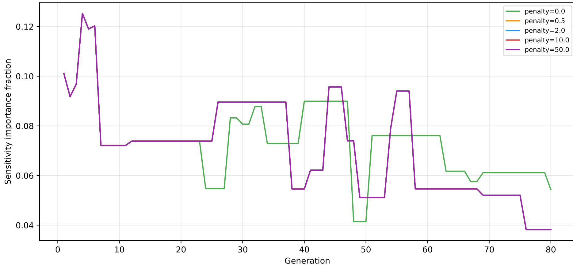
Cancellation module emergence over search time
