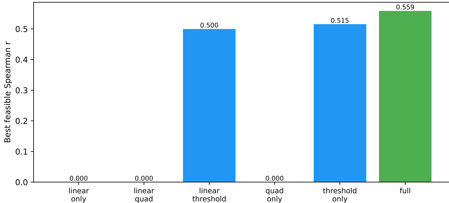
Representation family expressiveness
