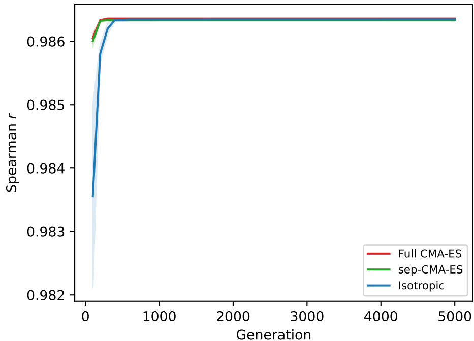
Prediction quality
