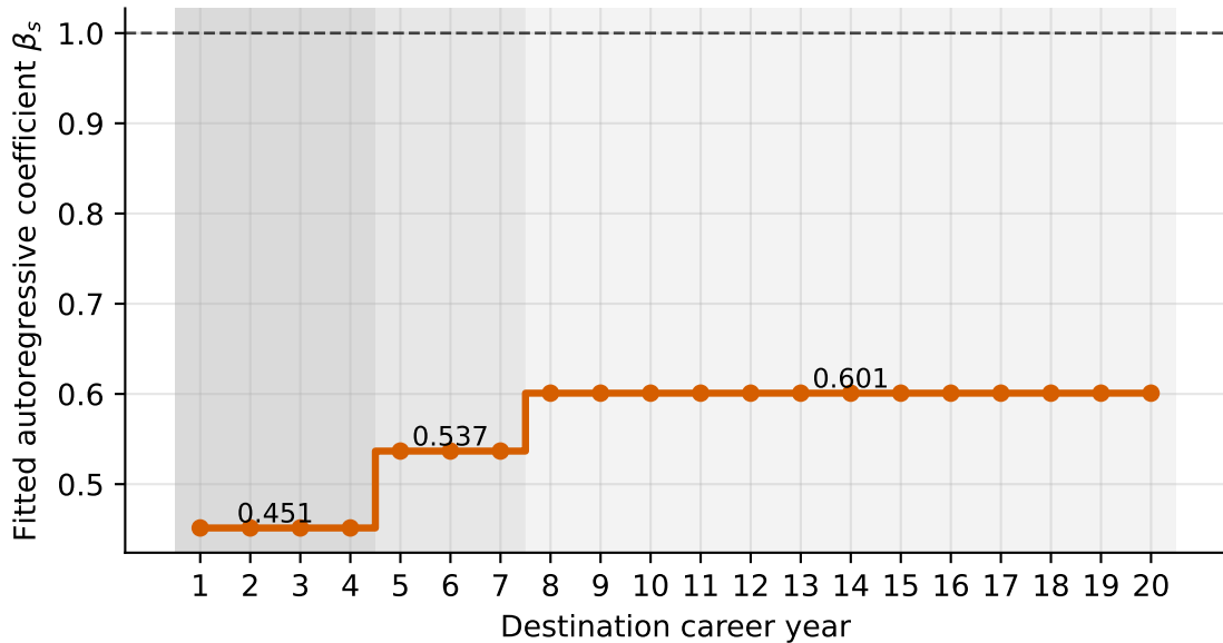
AR(1)-GRW-S: fitted autoregressive coefficient
