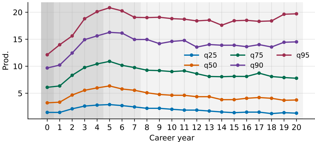
AR(1)-GRW-S prod. quantiles
