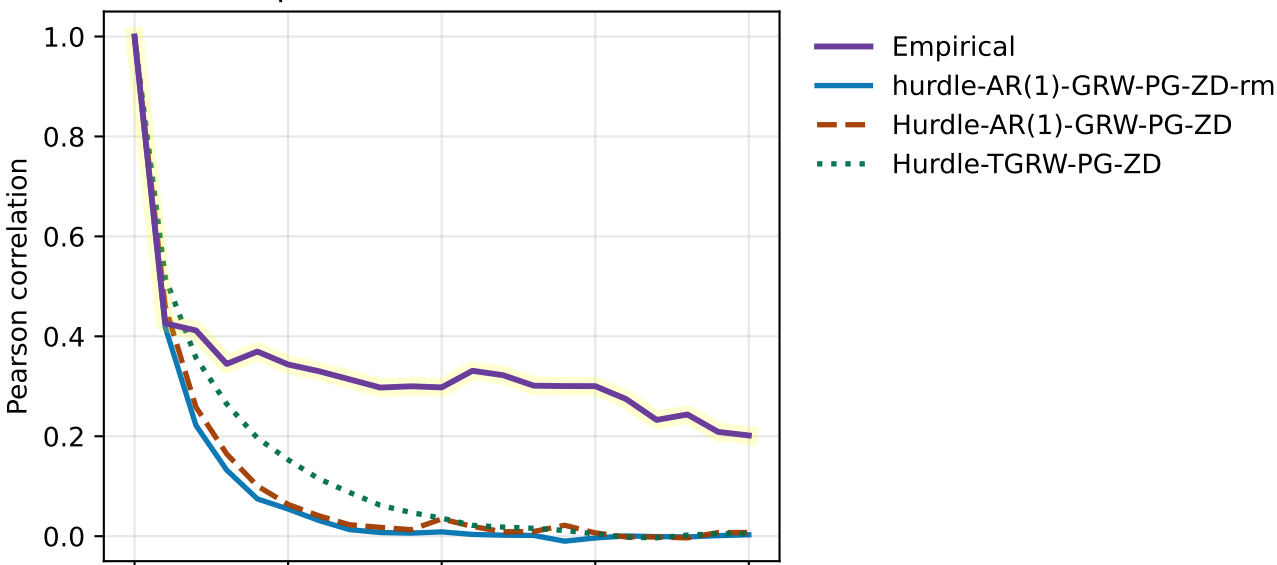
Empirical vs PG-ZD models
