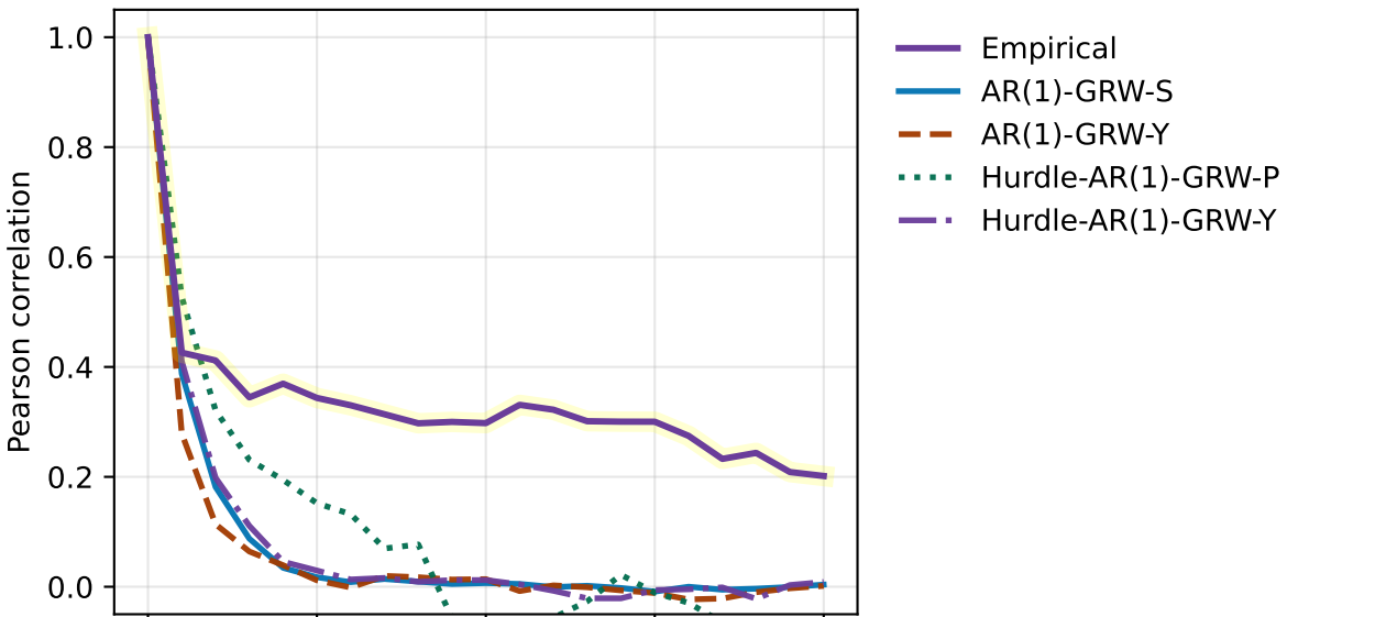
Empirical vs AR(1) models
