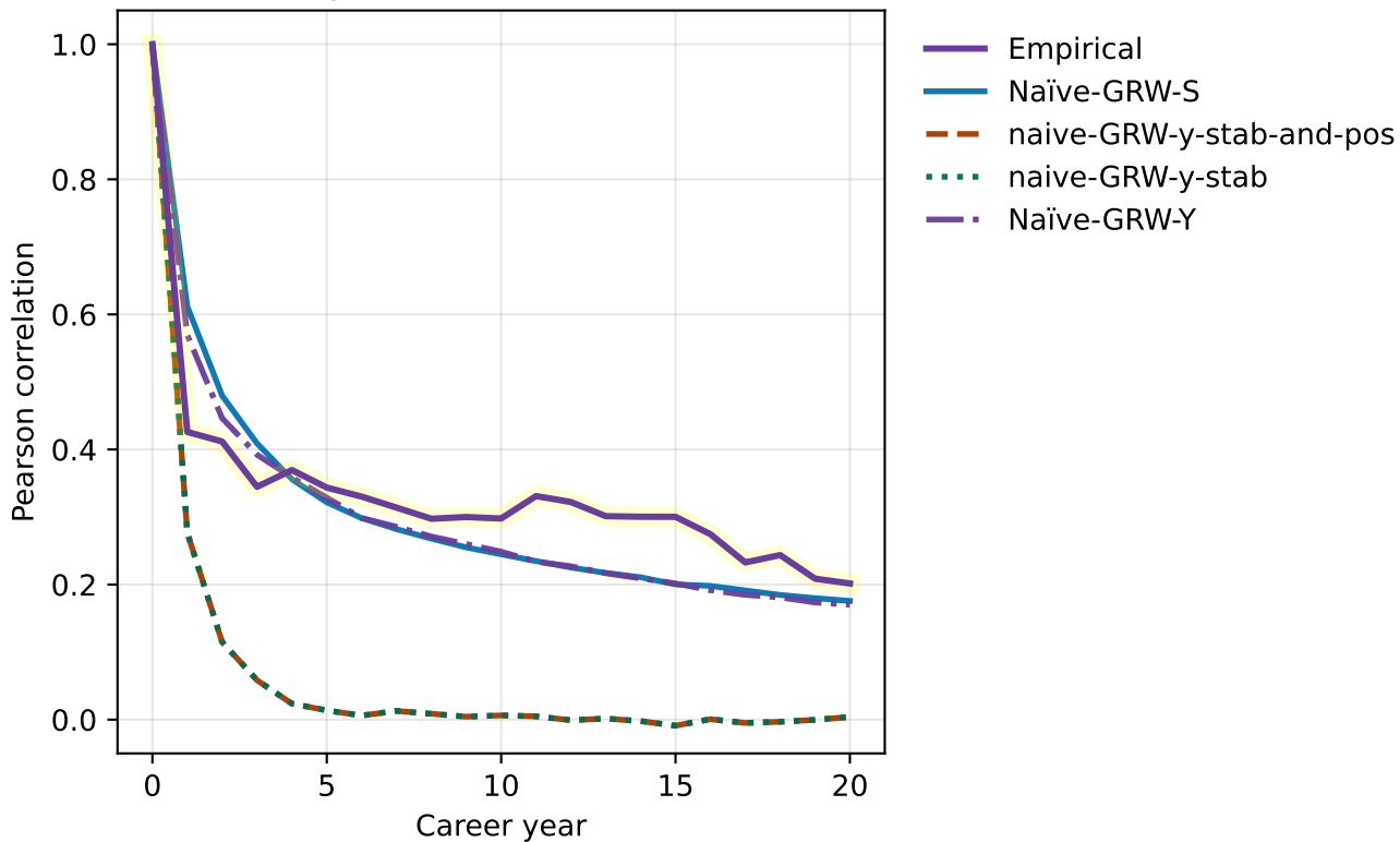
Empirical vs naïve models
