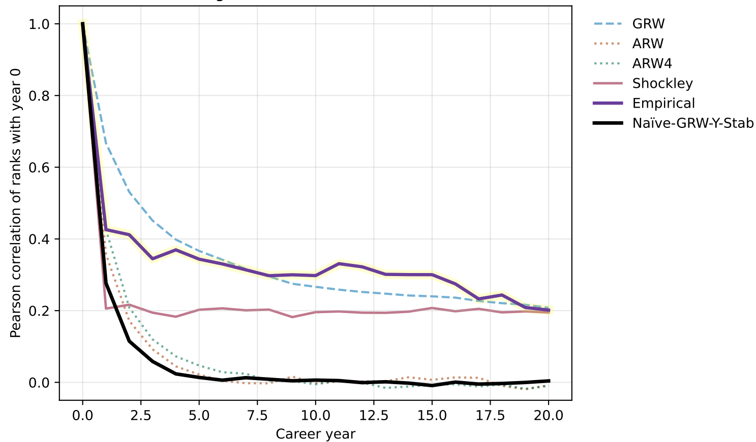
Rank mixing: Sam models + Naïve-GRW-Y-Stab
