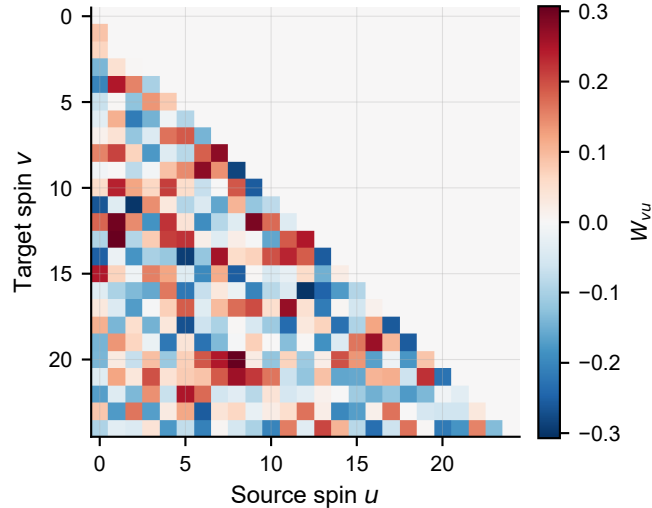
Square ( p = 4 ) ( 5 \times 5 , N = 25 )
