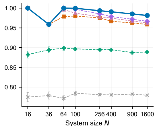
Hexagonal ( p = 6 ) \pm 1 bimodal couplings
