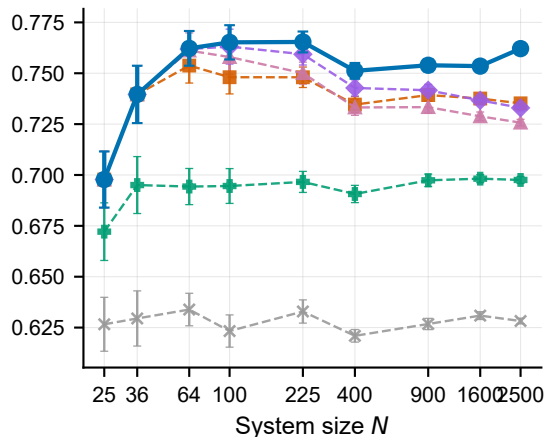
Square ( p = 4 ) \pm 1 bimodal couplings
