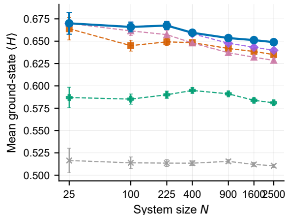
Triangular ( p = 3 ) \pm 1 bimodal couplings
