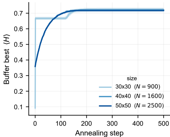
Triangular ( p = 3 ), \pm 1 bimodal couplings
