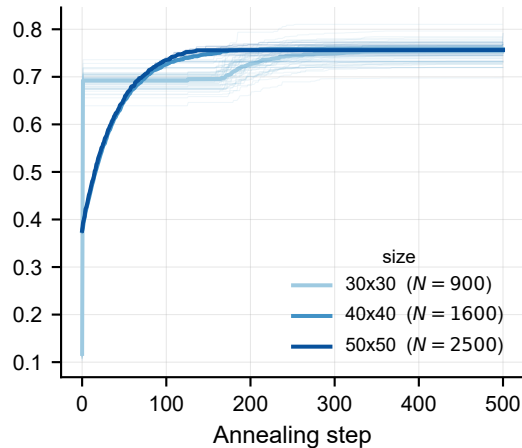
Square ( p = 4 ), Gaussian couplings
