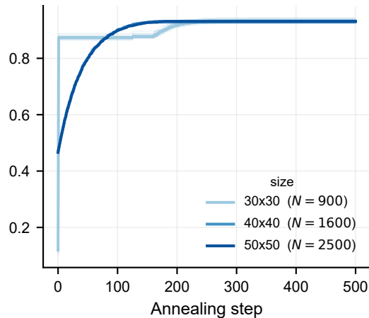
Square ( p = 4 ), \pm 1 bimodal couplings
