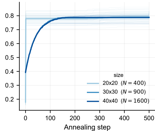
Hexagonal ( p = 6 ), Gaussian couplings
