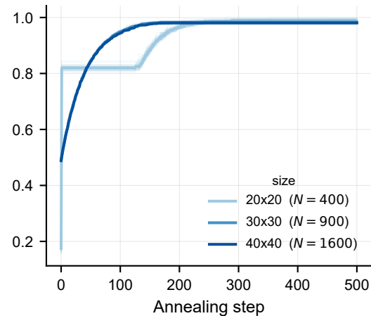
Hexagonal ( p = 6 ), \pm 1 bimodal couplings
