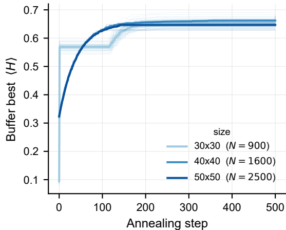
Triangular ( p = 3 ), Gaussian couplings
