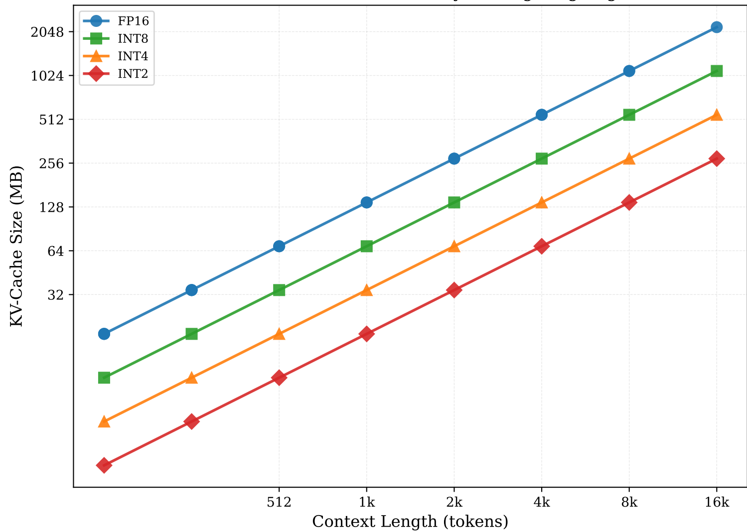
Mistral-7B: KV-Cache Memory Scaling (Log-Log)
