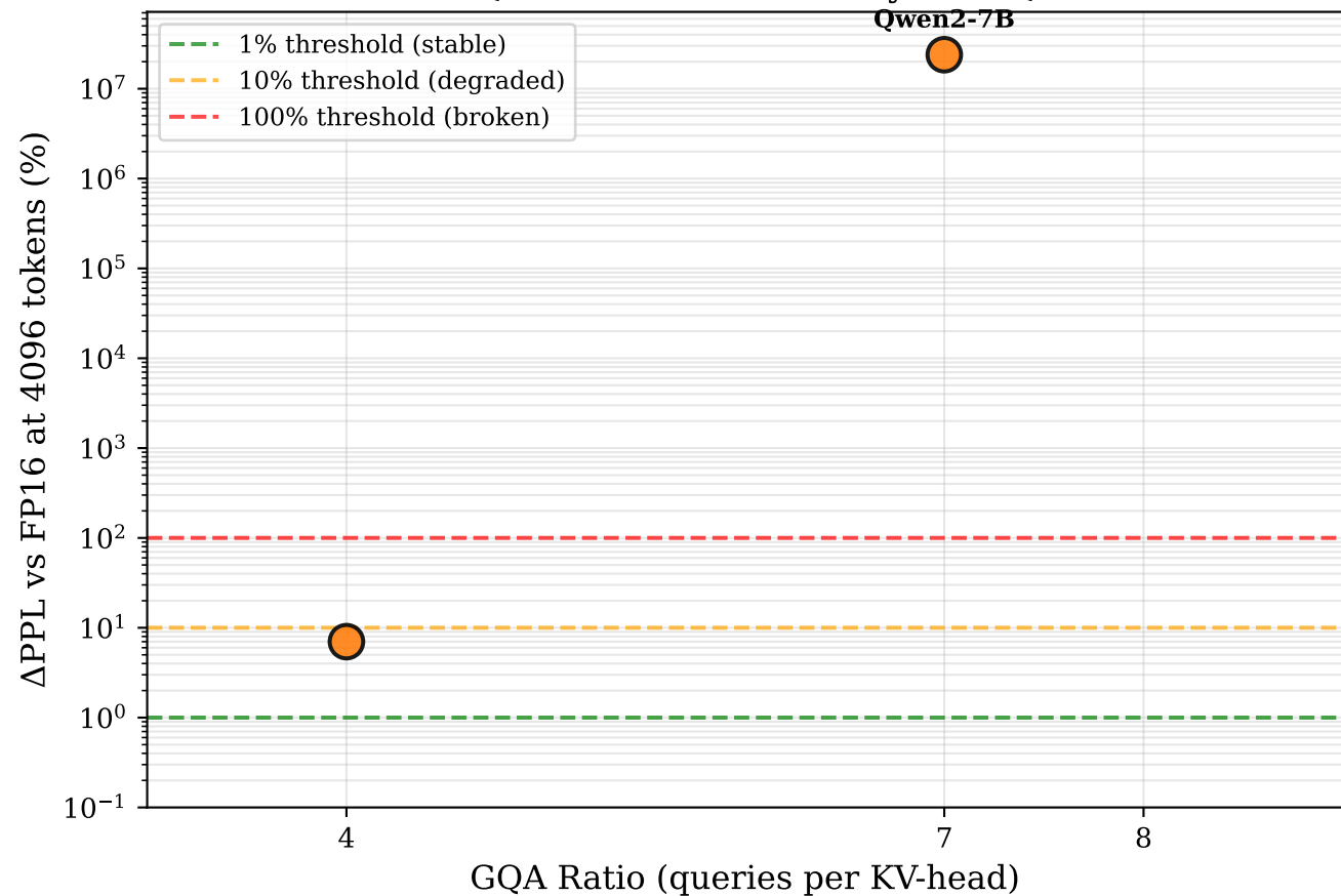
INT4 KV-Cache Quantization Sensitivity vs. GQA Architecture
