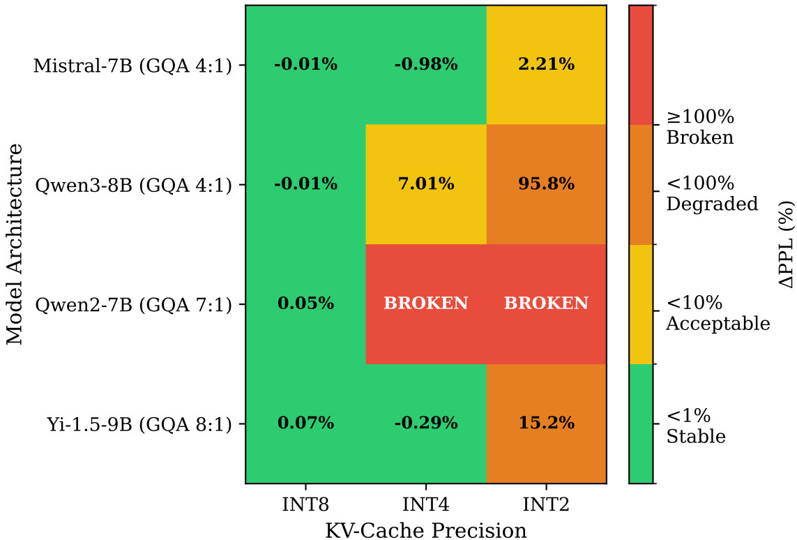
Quantization Stability at 4096 Tokens ( \Delta PPL vs FP16)
