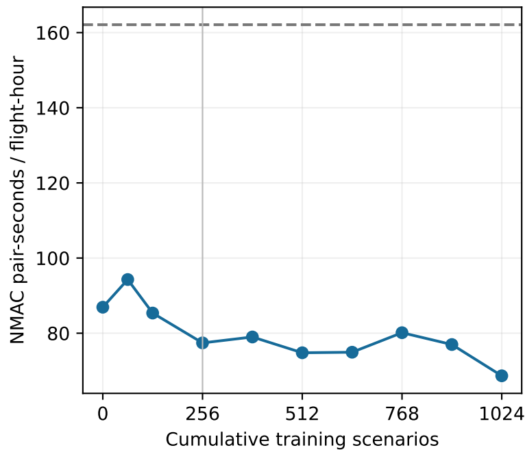
Unchanged2400s CPU PPO: 256 to 1024 scenarios One training seed; same12 DEV scenes; no held-out evaluation
