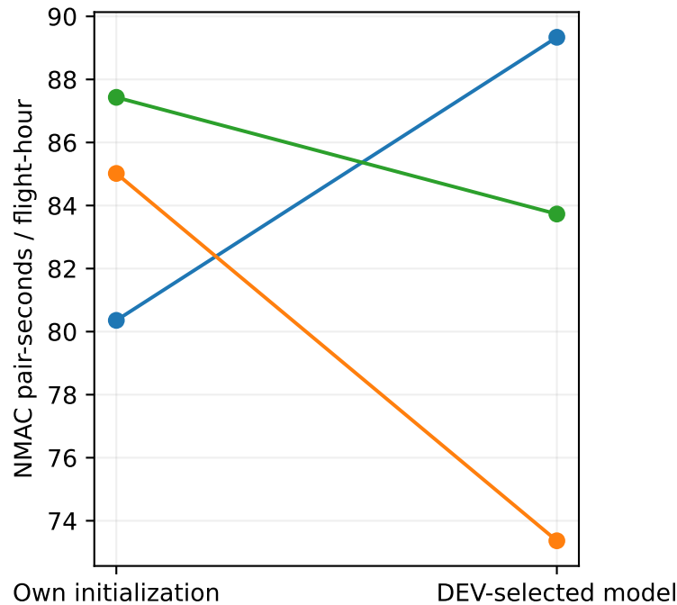
Independent training repeats on fixed24 external scenes
