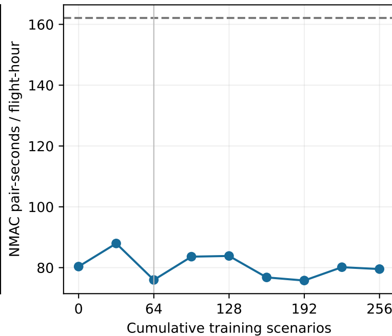
Unchanged CPU PPO continuation: 64 to 256 scenarios One training seed; same 12 development scenes; no held-out evaluation
