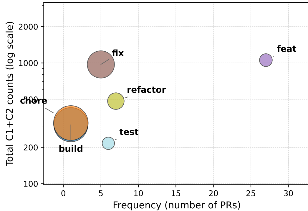
AI agents (47 outlier PRs)
