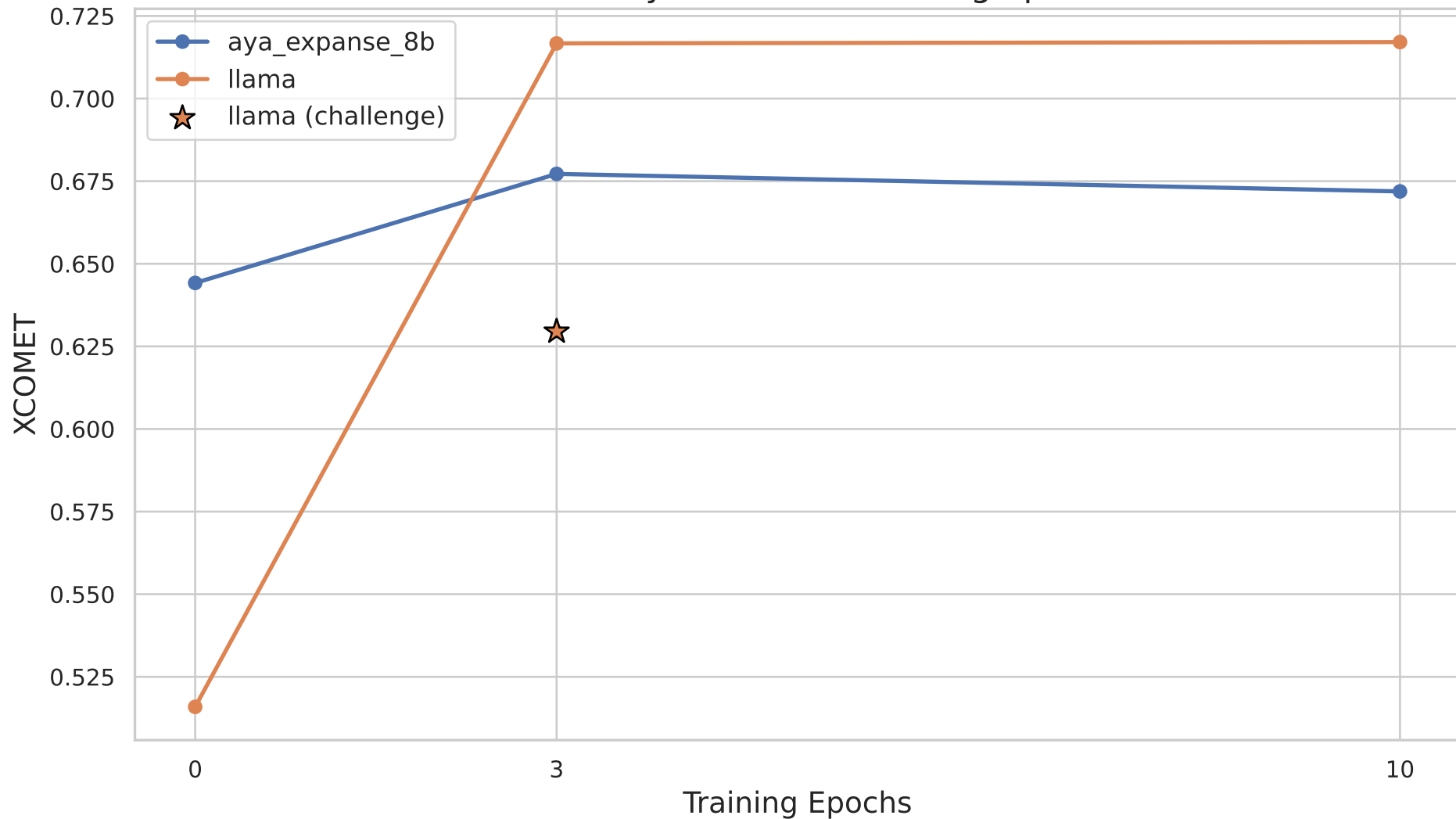
XCOMET by Model and Training Epochs
