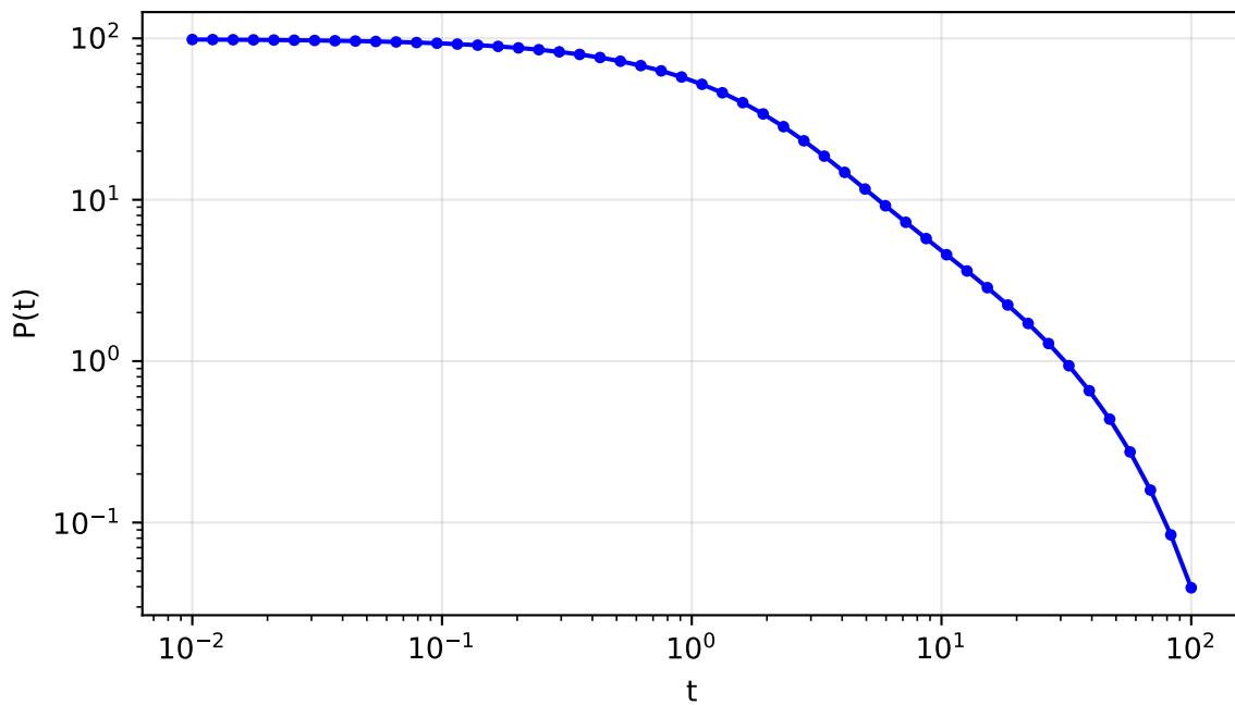
3D Random (expect d_s \sim 2-3 ) Heat Kernel
