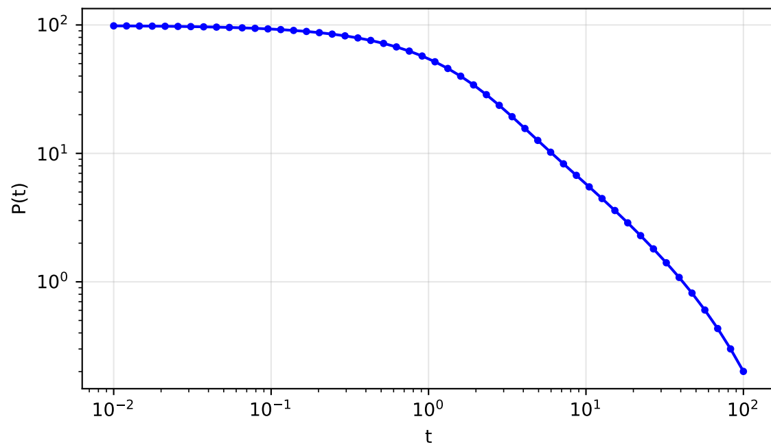
2D Sphere (expect d_s \sim 2 ) Heat Kernel
