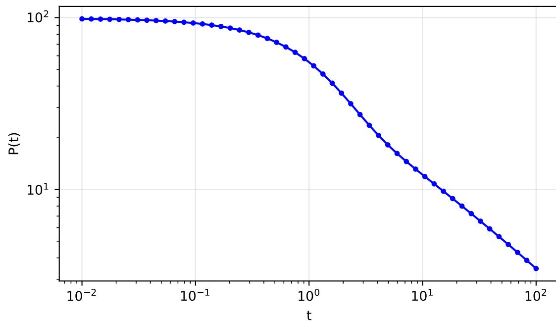
1D Filament (expect d_s \sim 1 ) Heat Kernel
