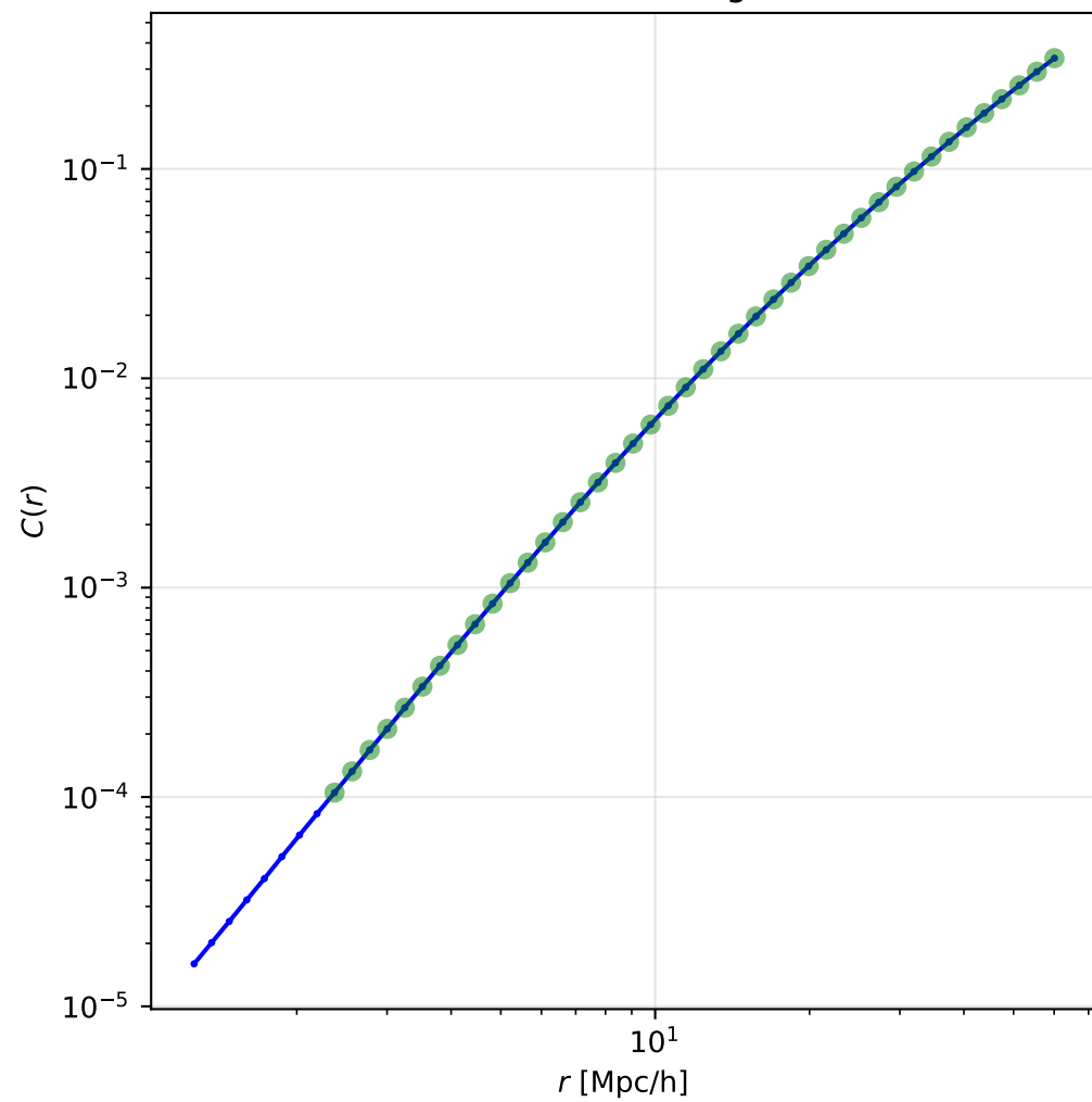
Correlation Integral
