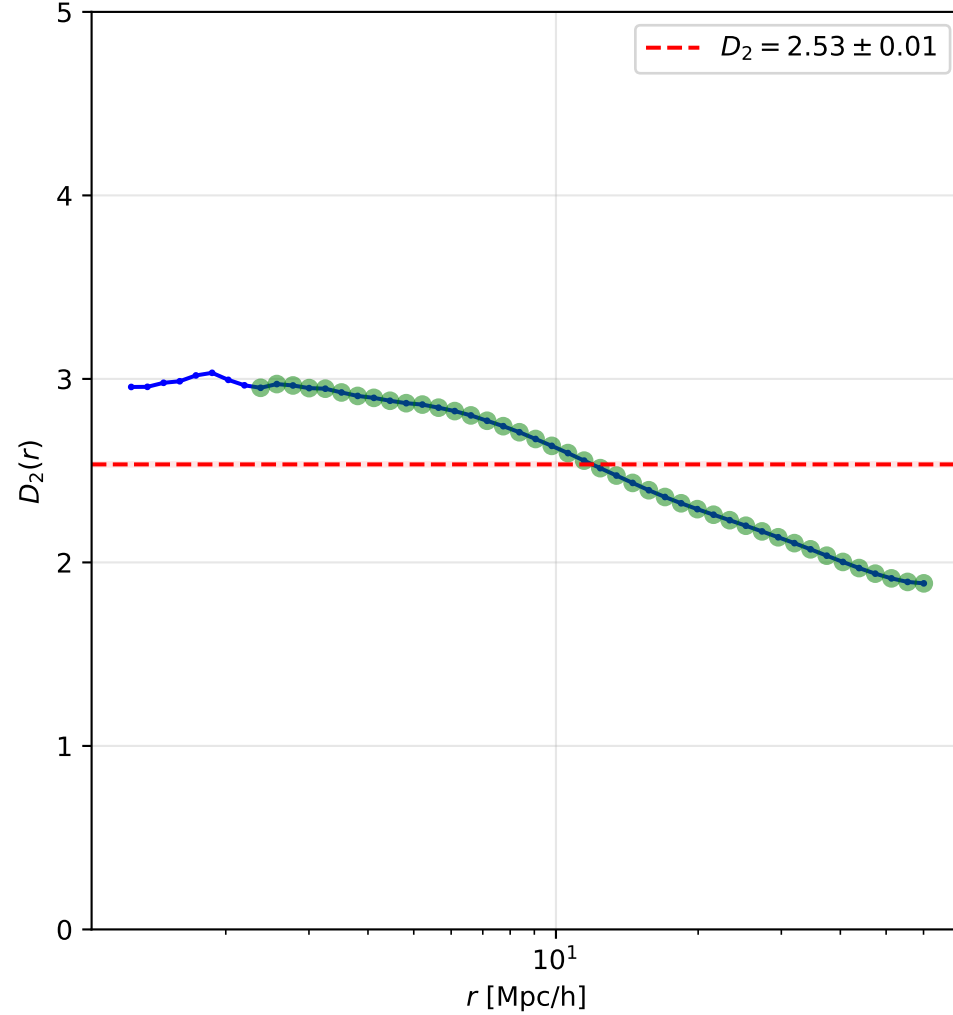
Correlation Dimension
