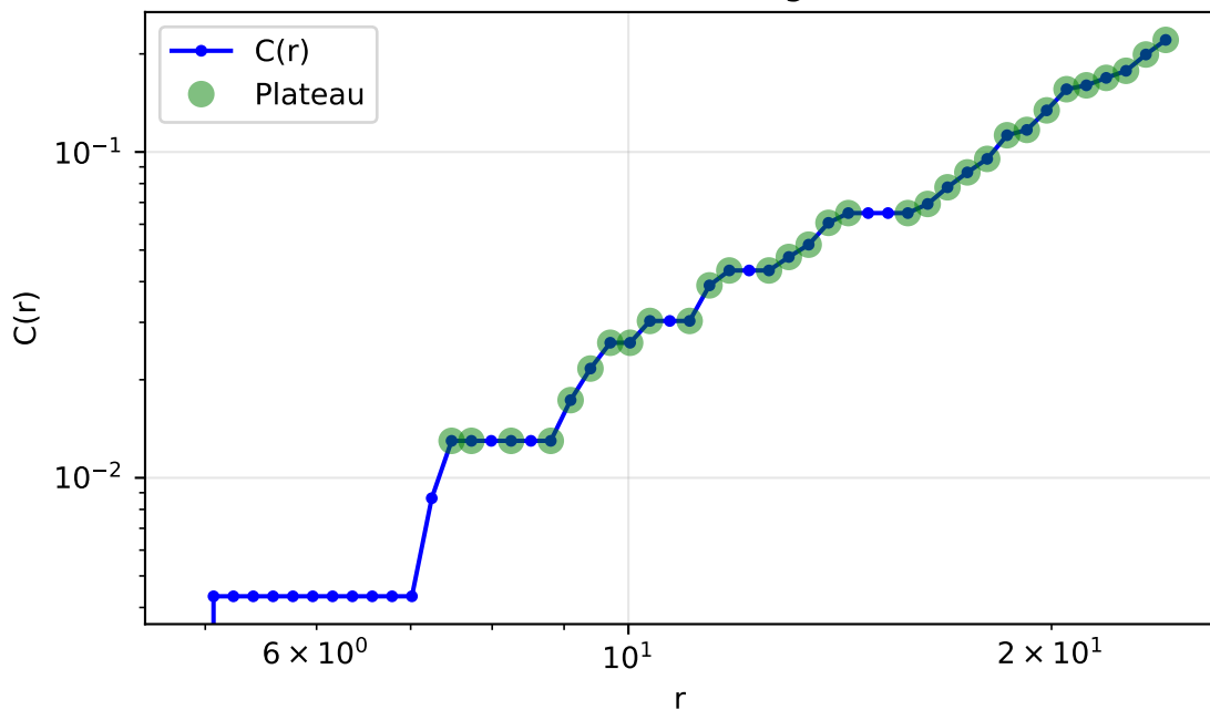
3D Random (expect D_2 \sim 3 ) Correlation Integral
