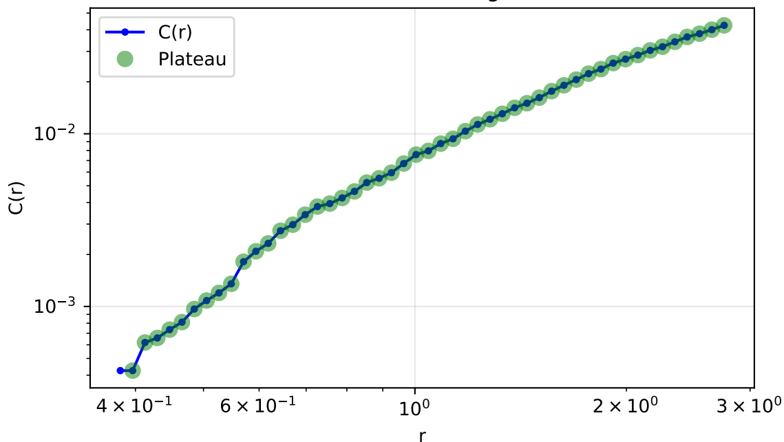
1D Filament (expect D_2 \sim 1 ) Correlation Integral
