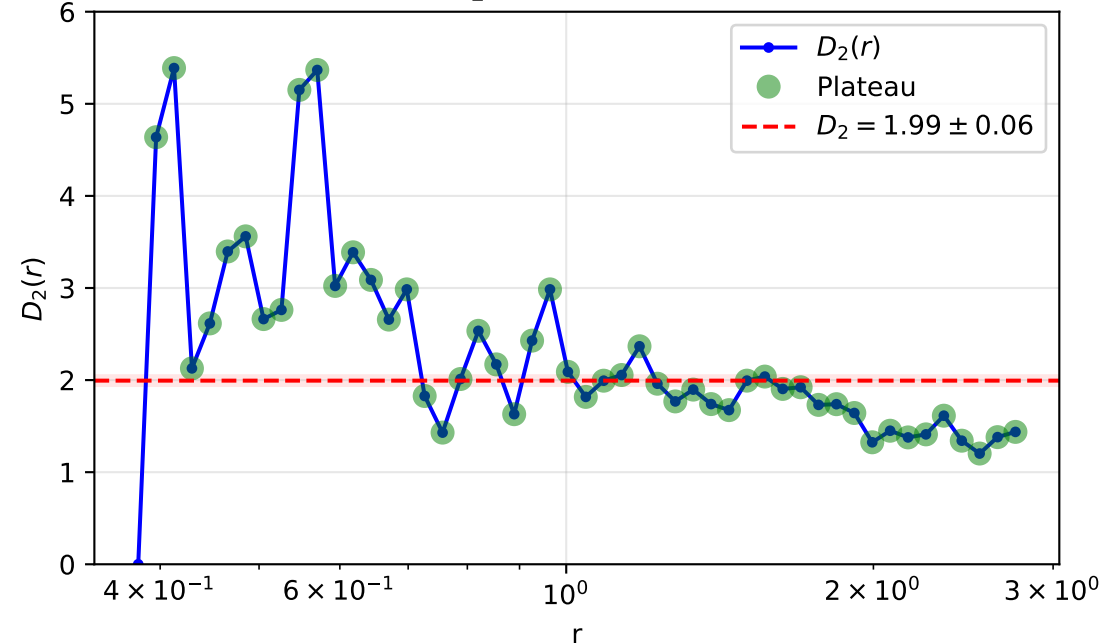
1D Filament (expect D_2 \sim 1 ) D_2 = 1.99 \pm 0.06
