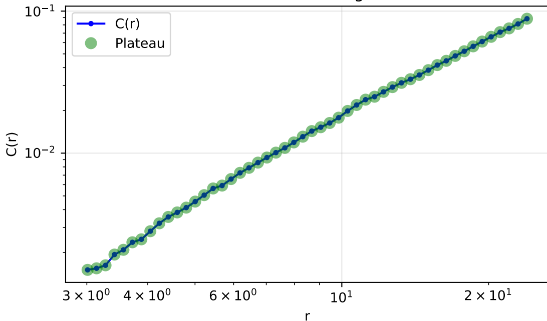
2D Surface (expect D_2 \sim 2 ) Correlation Integral
