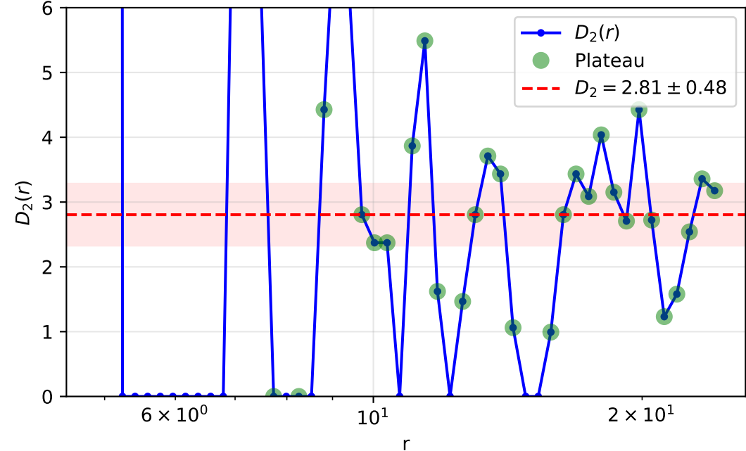
3D Random (expect D_2 \sim 3 ) D_2 = 2.81 \pm 0.48
