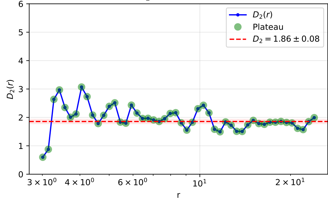
2D Surface (expect D_2 \sim 2 ) D_2 = 1.86 \pm 0.08
