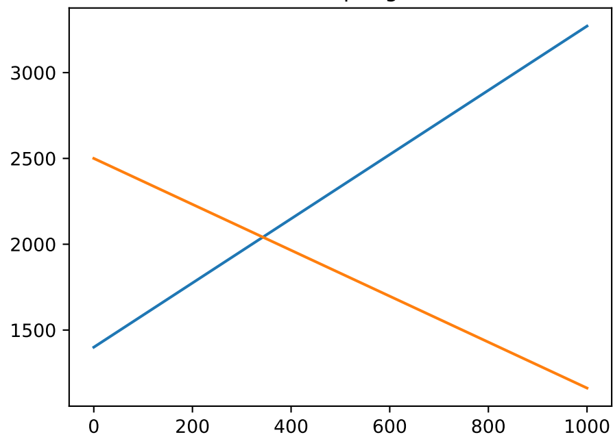
Toxic Sponge
