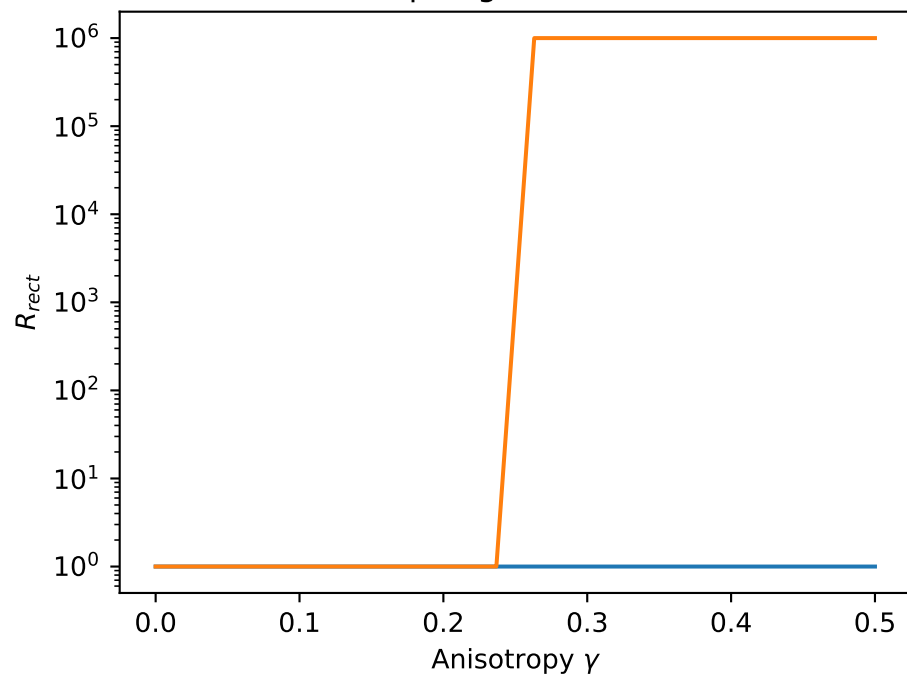
Topological Diode
