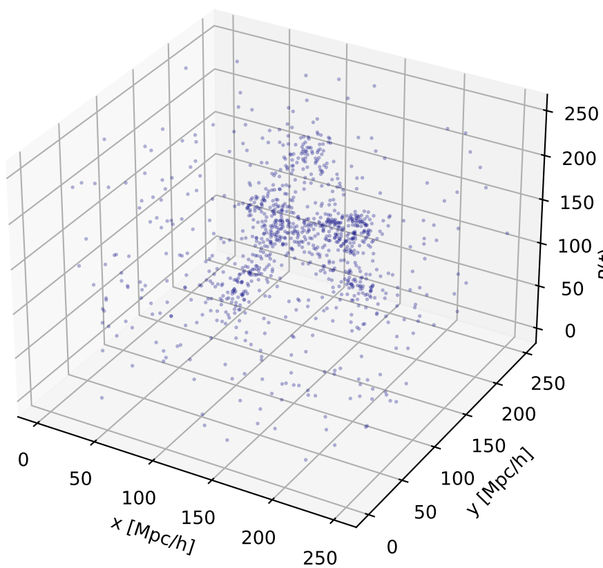
Halo Positions (N=2000)
