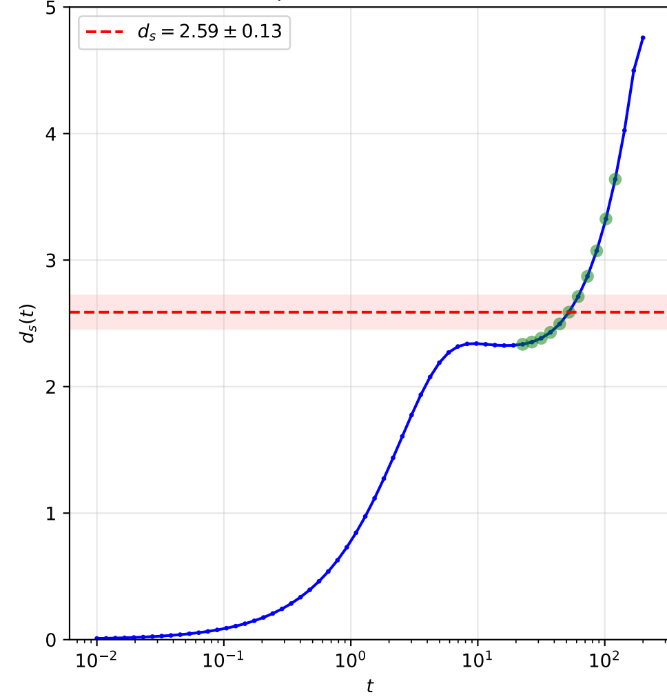
Spectral Dimension
