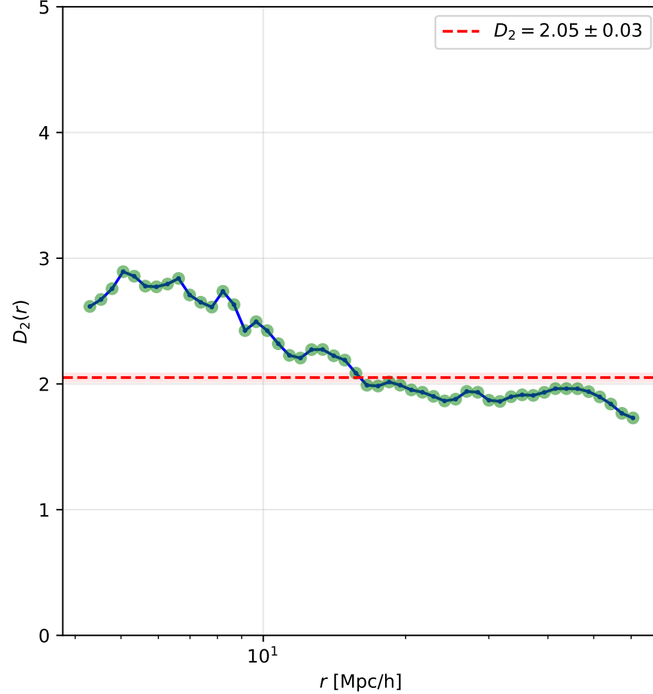
Correlation Dimension
