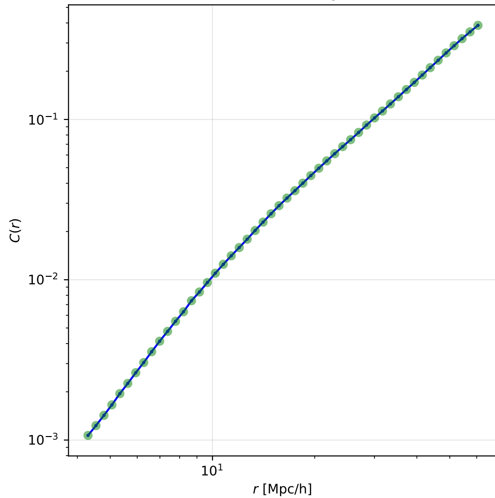
Correlation Integral
