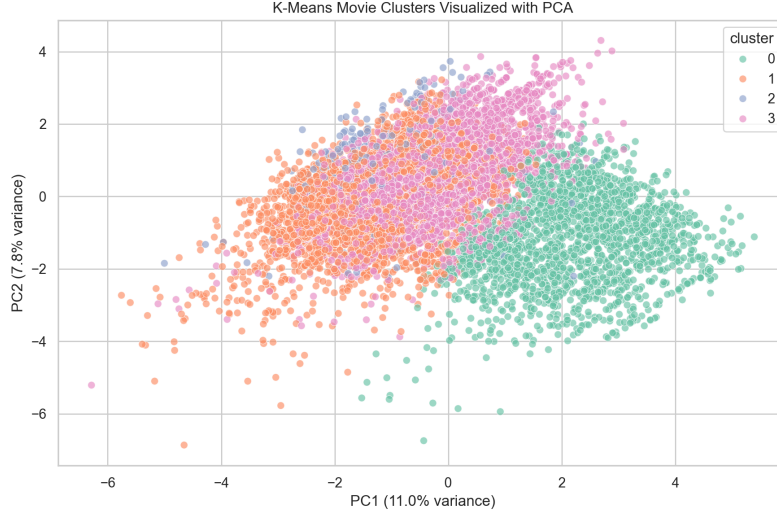
Figure 4: PCA visualization of K-Means movie clusters.
