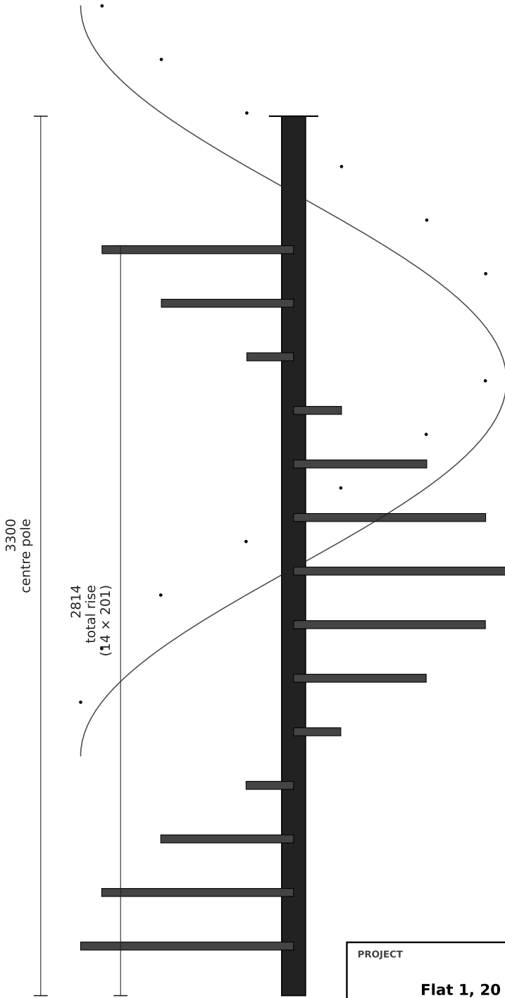
ELEVATION (developed) Treads laid out side-projected from centre pole
