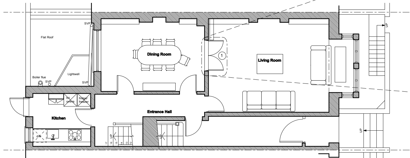
7 Proposed Plans Scale: 1:100
