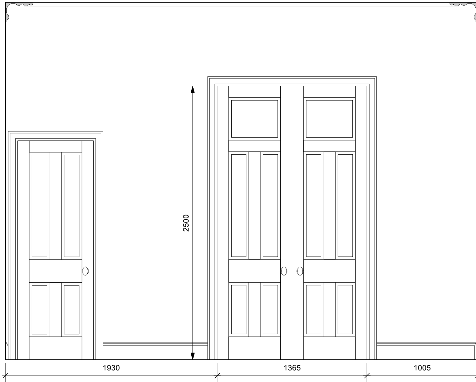
11 Proposed Door Elevation from Living Room Scale: 1:20
