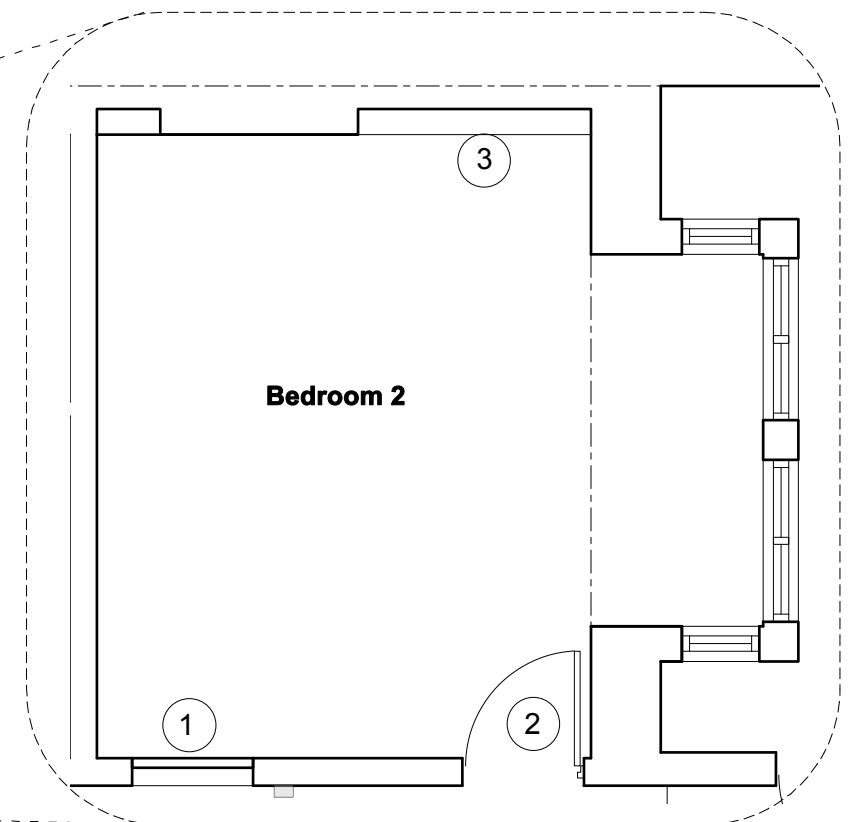
4 Proposed Bedroom 2 Plan Scale: 1:50
