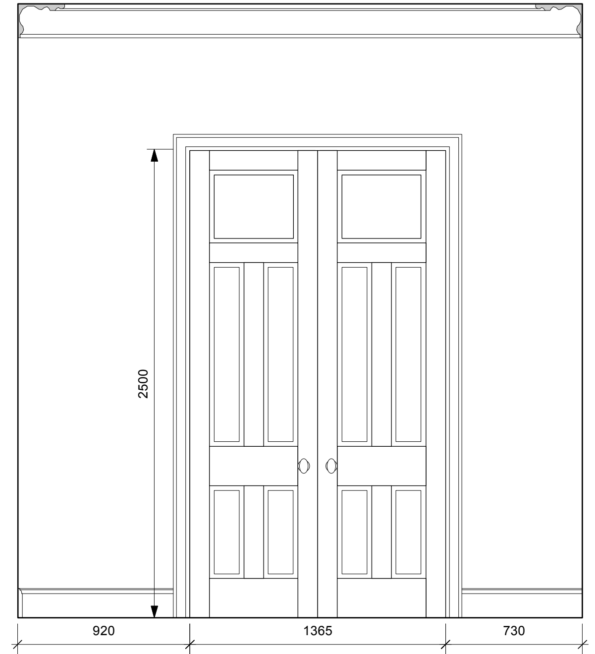
12 Proposed Door Elevation from Sitting Room Scale: 1:20
