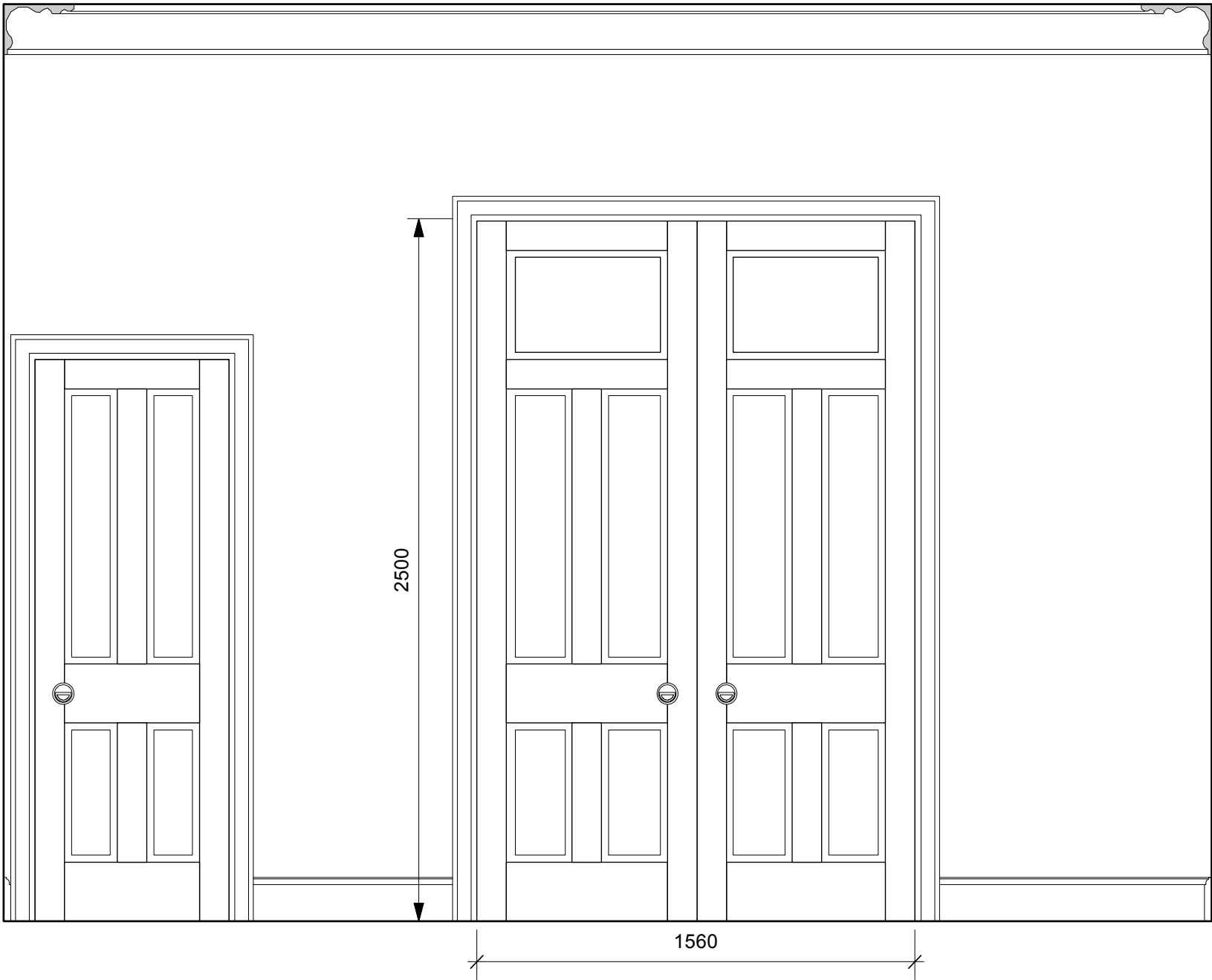
9 Previously Approved Door Elevation from Living Room Scale: 1:20
