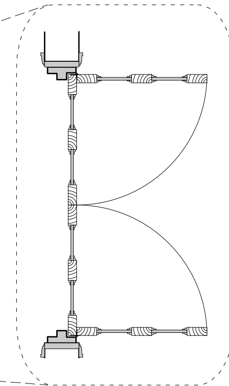
8 Proposed Door Detail Scale: 1:20
