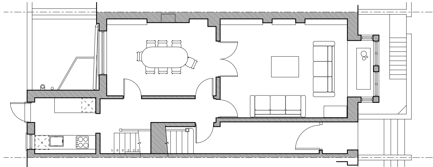
6 Previously Approved Groundfloor Plan Scale: 1:20
