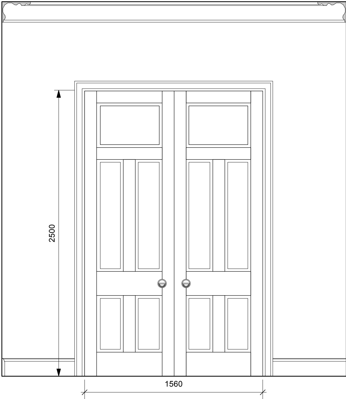
10 Previously Approved Door Elevation from Sitting Room Scale: 1:20
