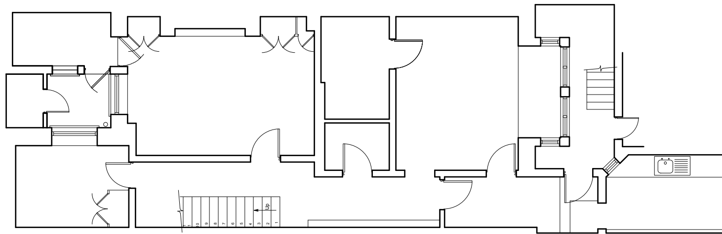
1 Existing Basement Plan Scale: 1:100
