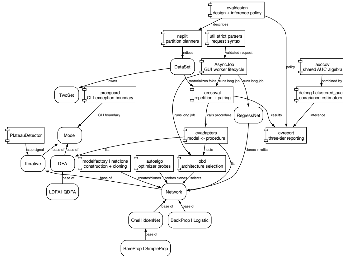
Figure 12.1: Object design
