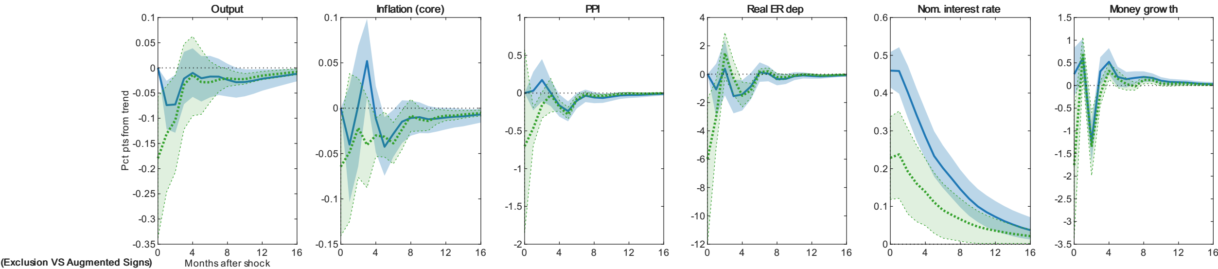
Figure 9: Comparison of Identifying Assumptions — VAR w/ Exo
