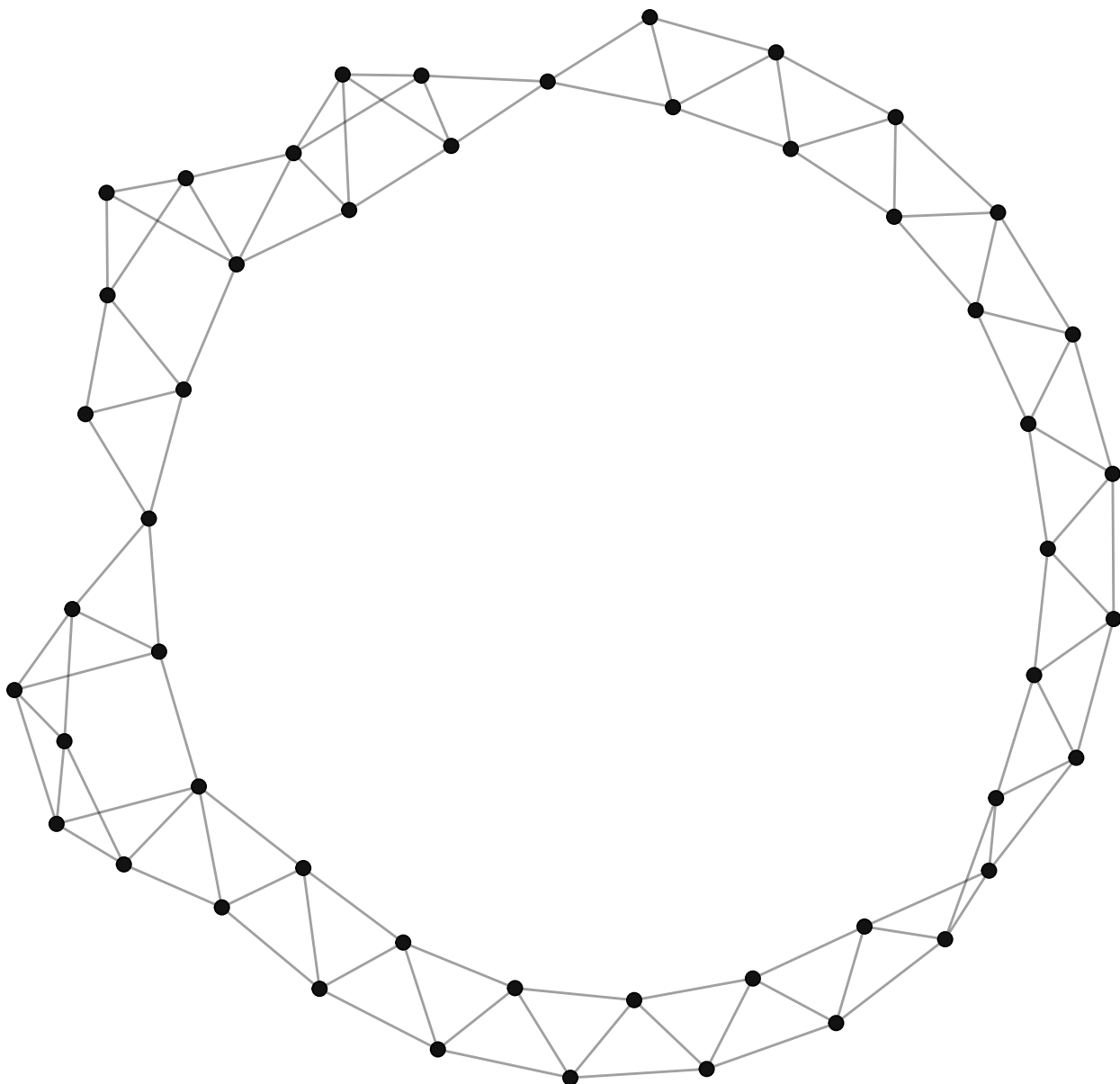
Smallworld 1 graph
