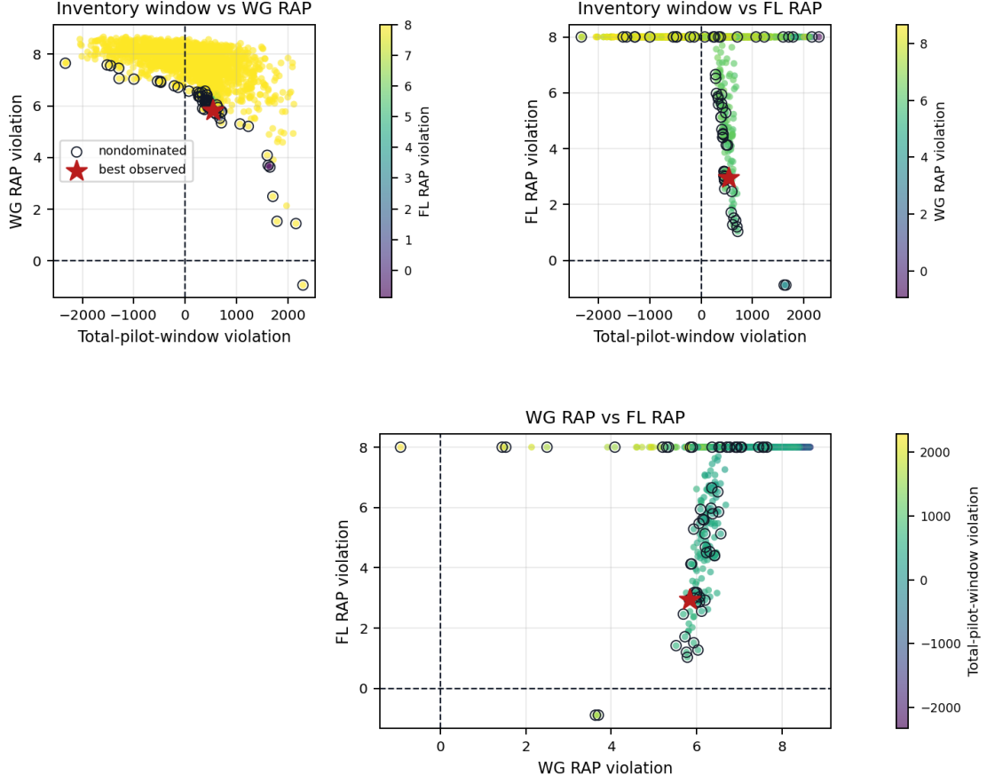
Figure 6: Three direct-physics views of the current-bound constraint trade space. Each panel shows the same evaluated policies with two violations on the axes and the third violation encoded by color. Lower-left is better; dashed lines mark zero violation. Open circles mark policies that are nondominated over total-pilot-window, WG RAP, and FL RAP violations, and the red star marks the best observed policy.
