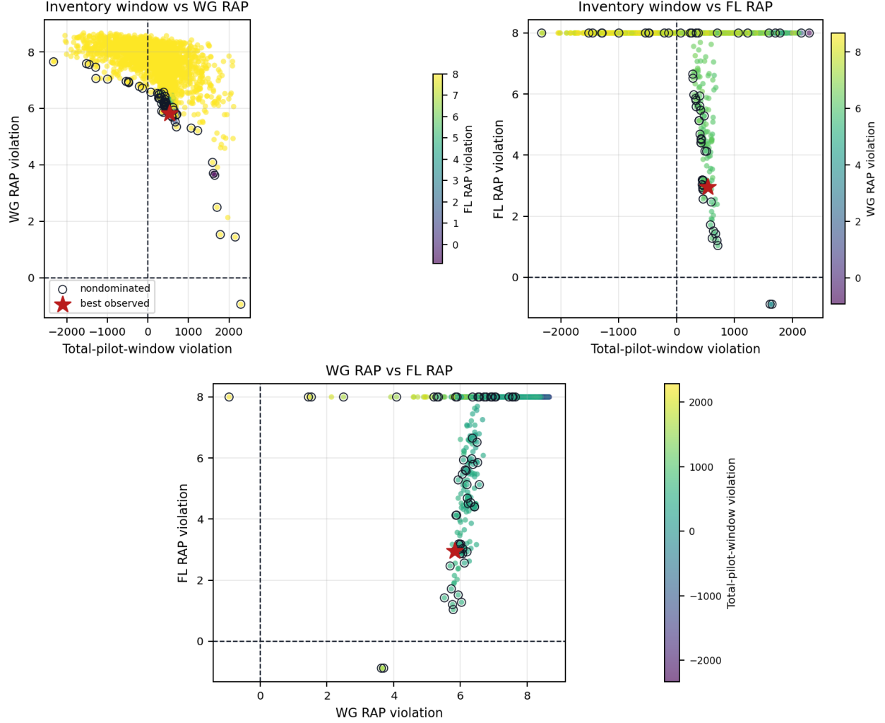
Figure 6: Three direct-physics views of the current-bound constraint trade space. Each panel shows the same evaluated policies with two violations on the axes and the third violation encoded by color. Lower-left is better; dashed lines mark zero violation. Open circles mark policies that are nondominated over total-pilot-window, WG RAP, and FL RAP violations, and the red star marks the best observed policy.
