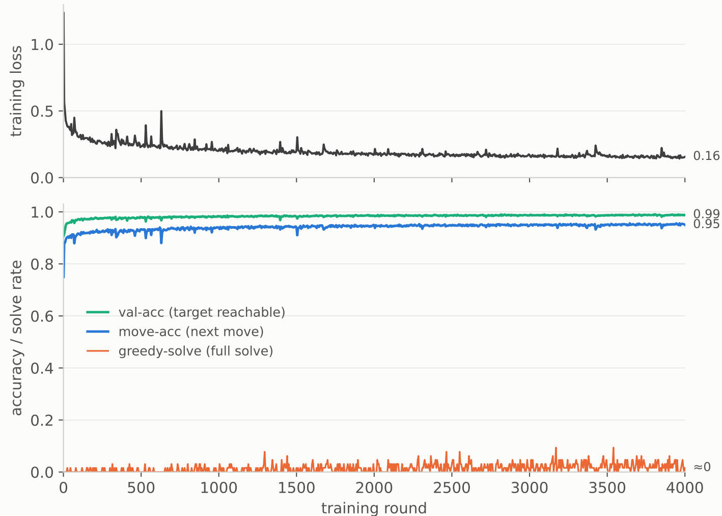
Learning process — N=16 (depth-16 dilated CNN, pop-conditioned, 4000 rounds)
