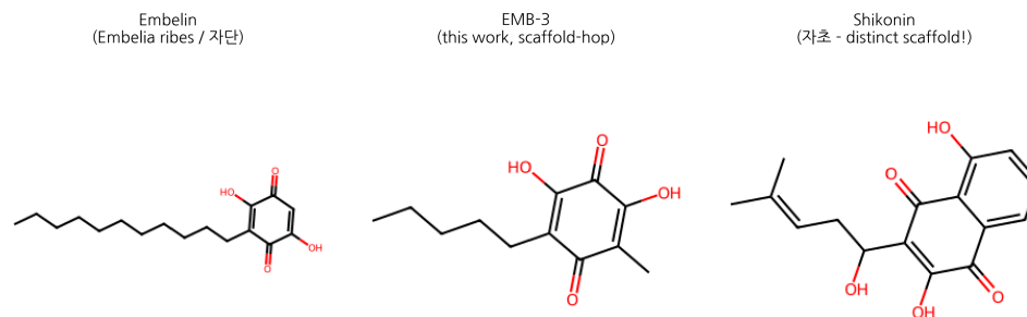
Figure 1: Embelin / EMB-3 / Shikonin structures
