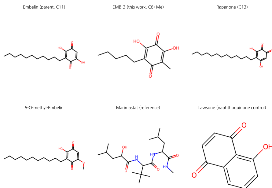
Figure 1: Embelin scaffold-hop SAR structures
