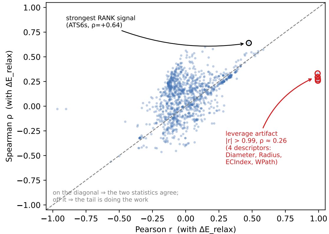
A Every descriptor: rank vs product-moment
