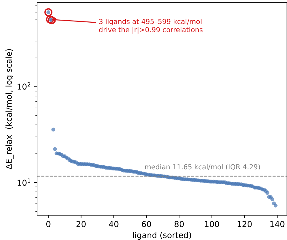
B Why: the dependent variable is heavy-tailed
