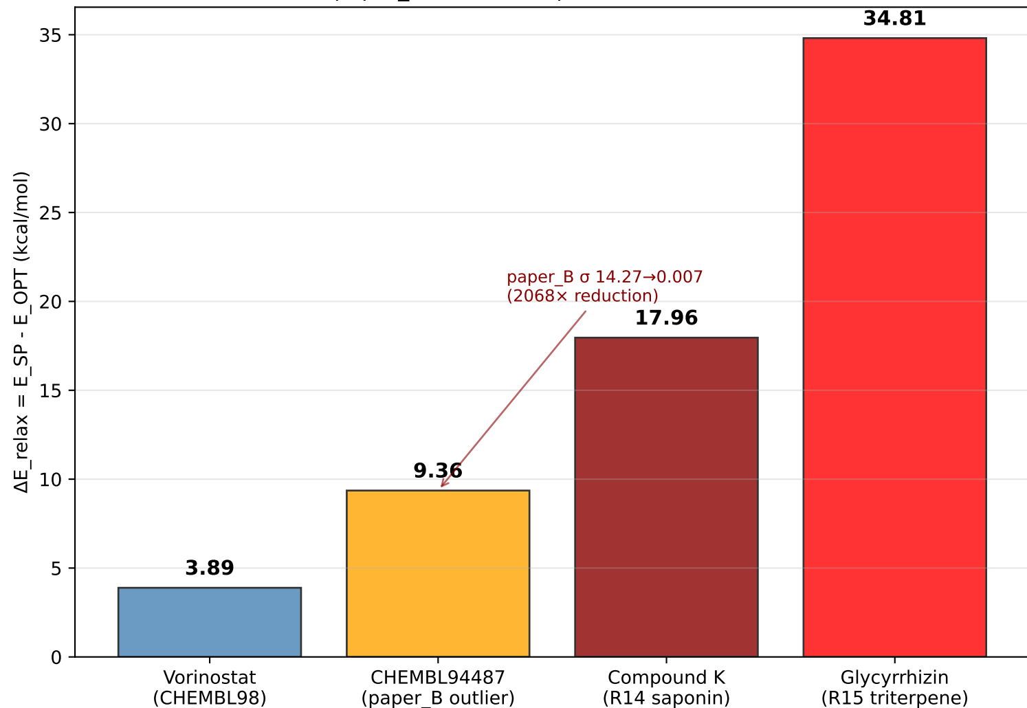
Figure 3. xtb GFN2 conformational energy refinement (paper_B \sigma outlier expansion candidates)
