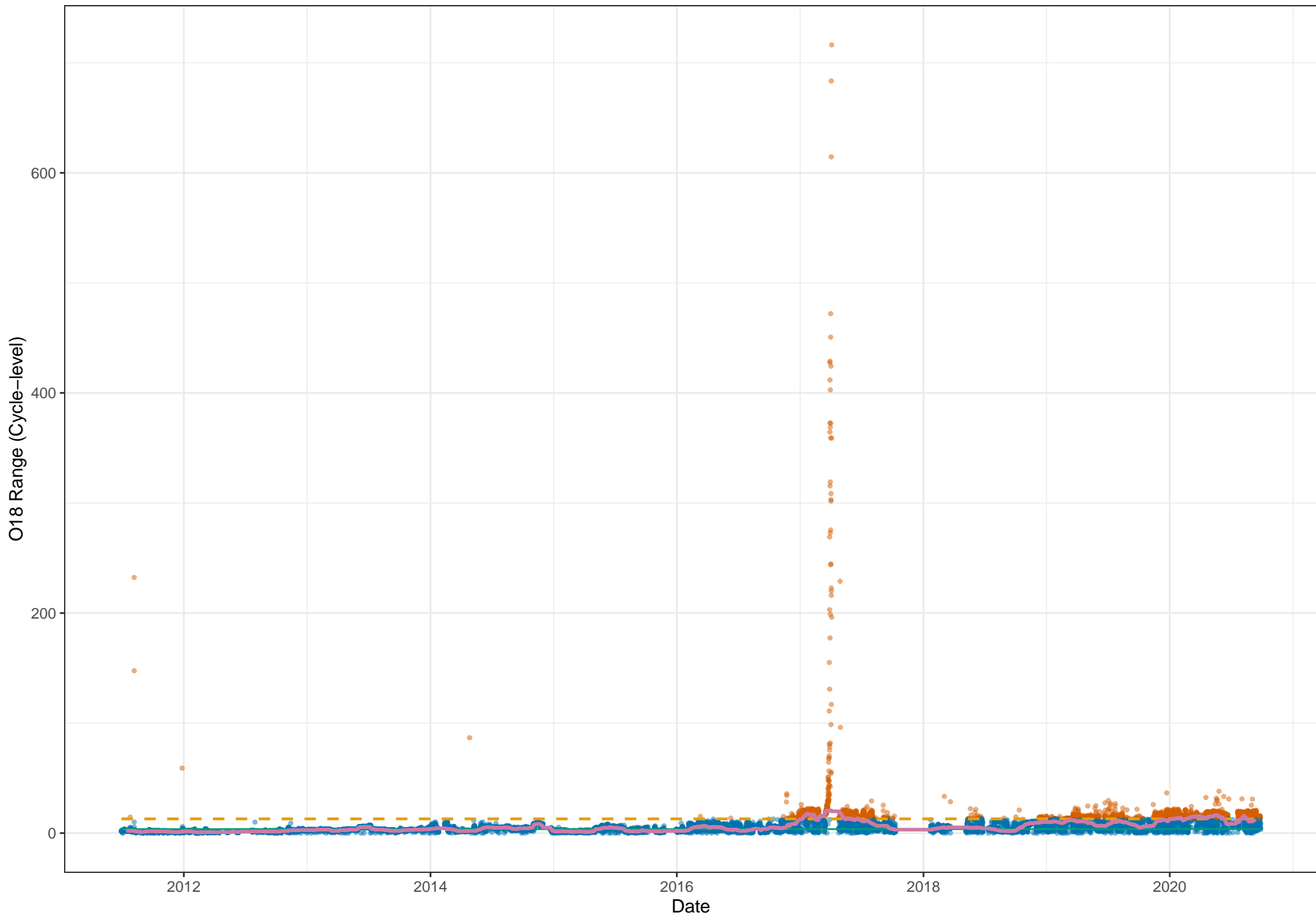
O18 Range Variability Time Series: More Sensitive to Extremes
