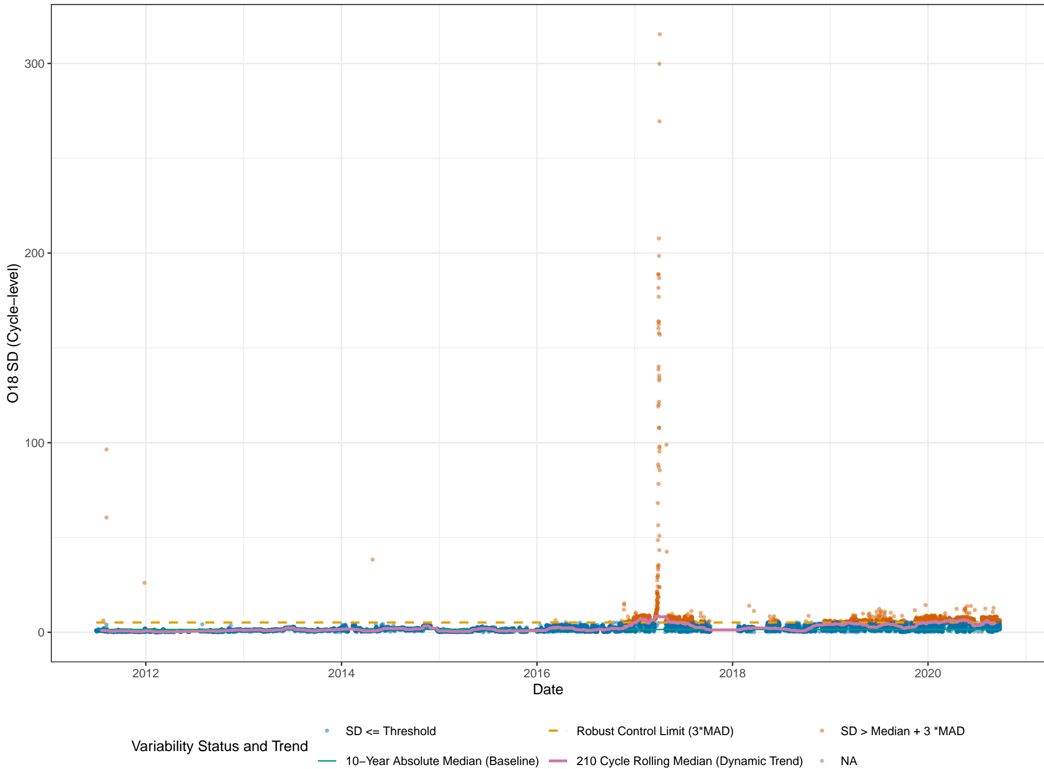
O18 SD Variability Time Series: Absolute Fluctuation and Dynamic Trend
