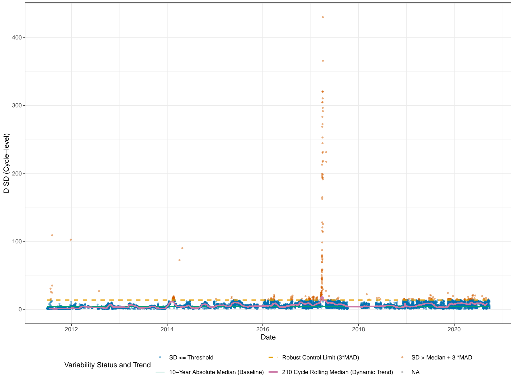
D SD Variability Time Series: Absolute Fluctuation and Dynamic Trend
